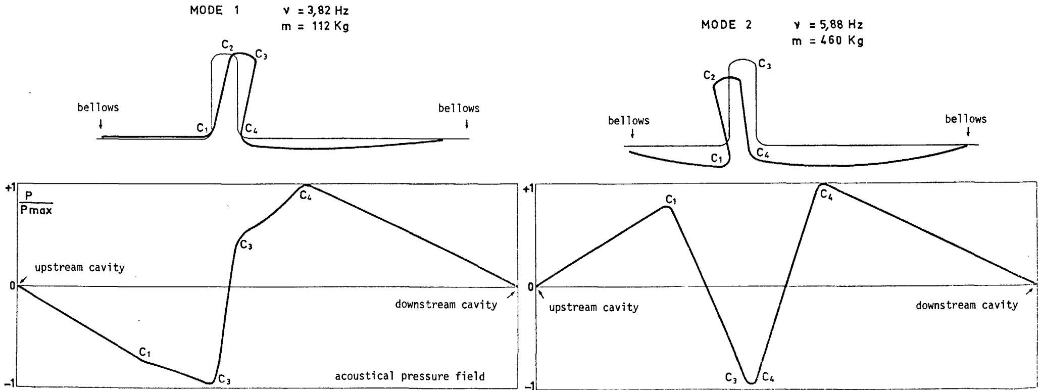
FIG. 2 COMPUTED MODAL SHAPES
