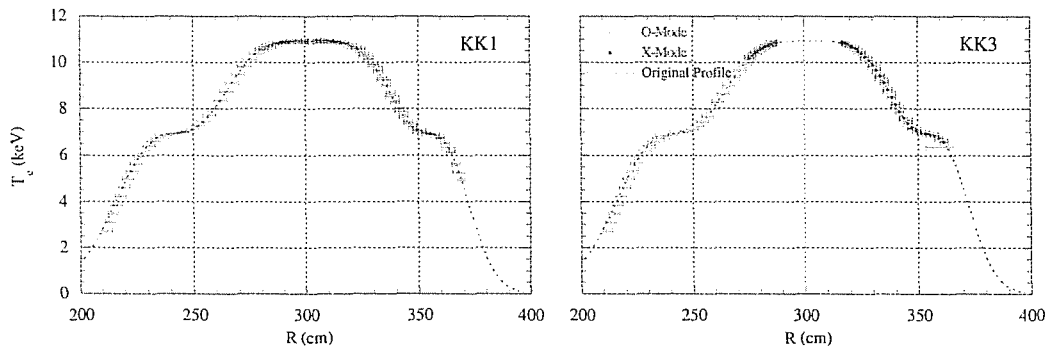
Figure 13: Simulated electron temperature profiles for KK1 and KK3 diagnostics with the original profile for the shot #47413. The error bars correspond to the spatial resolution of Fig. 12.
