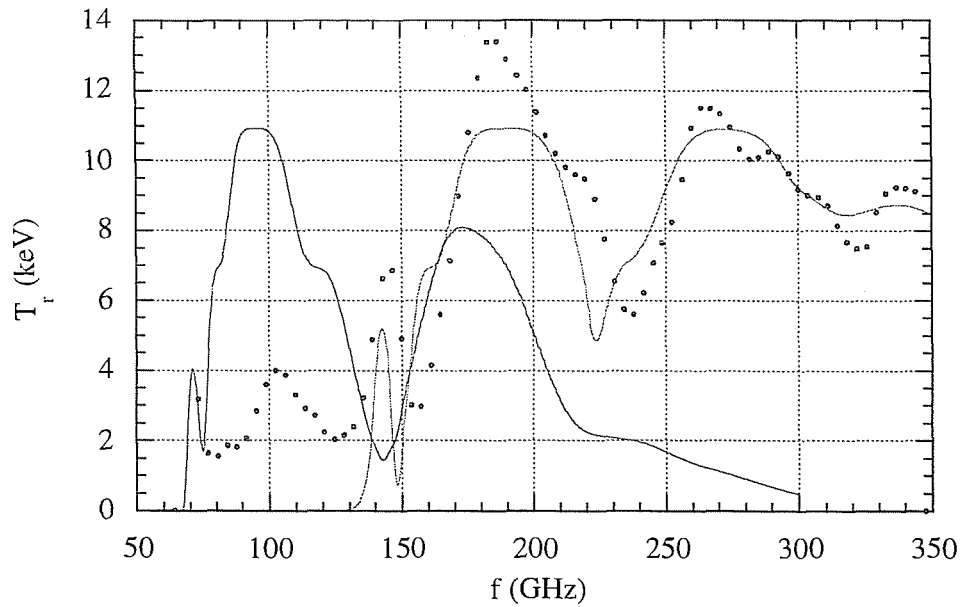
Figure 6: Electron cyclotron emission spectra, in temperature units, for the shot #47413 obtained with the KK1 Michelson interferometer and simulated with the ray tracing code for the first harmonic O-mode and second harmonic X-mode.
