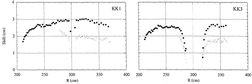
Figure 15: Distance between the cold resonance position and the average origin of the emission obtained for the KK1 (left) and KK3 (right) systems for the equivalent major radius deduced from the flux surfaces and the O-mode (close symbols) and X-modes (open symbols), and the conditions of the shot #47413.
