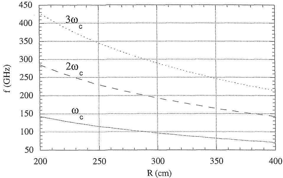
Figure 10: Radial dependence of the different cyclotron harmonics for the shot #47413.
