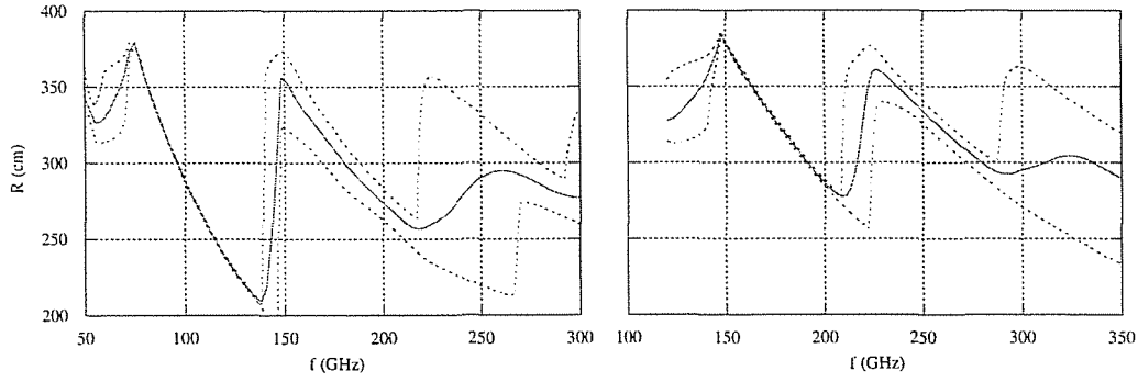
Figure 9: Average position \langle R \rangle (solid), R^{\min} and R^{\max} (dotted) versus frequency for the O-mode (left) and X-mode (right) ECE of shot # 47413 simulated with the ray tracing code.
