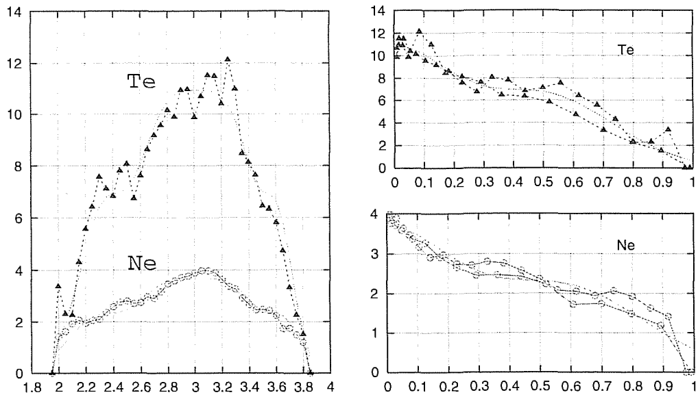
Figure 4: The same as in Fig. 3 but with the profiles shifted by 10 cm in major radius.
