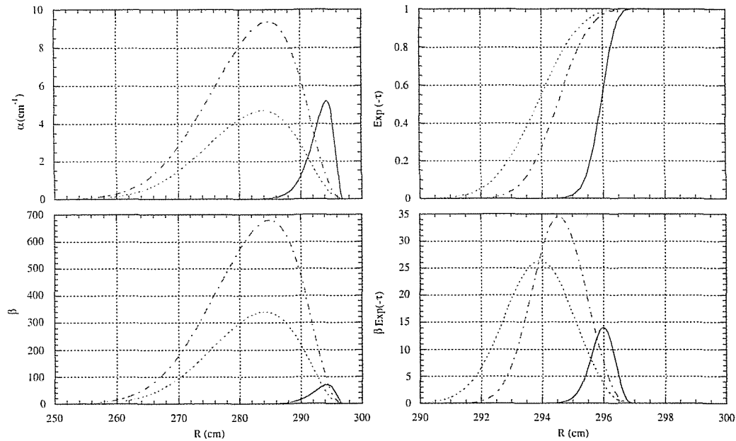
Figure 7: From top to bottom. Local absorption, emission, transmission and emitting coefficients versus the major radius for the parameters of Table 2: cases 1 shot #47413 (dotted), 2 (solid), and 3 (dashed).
