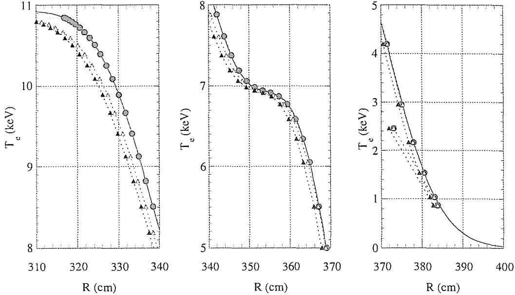
Figure 14: Original (solid) and simulated electron temperature profiles for KK3, for the equivalent major radius (full circles), major radius (full triangles) and major radius for the cold resonance position (open triangles) corresponding to the conditions of Fig. 13 and the X-mode emission.
