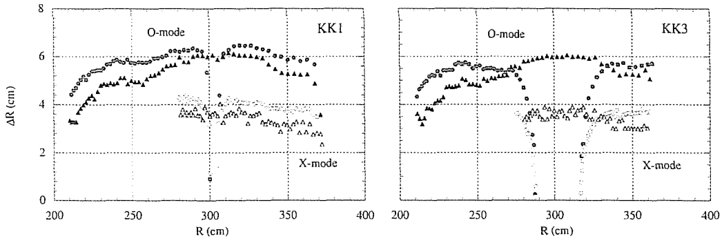
Figure 12: Spatial resolution, \Delta R , obtained for the KK1 (left) and KK3 (right) systems for the geometrical major radius (triangles) and the equivalent major radius deduced from the flux surfaces (circles) and the O-mode (close symbols) and X-modes (open symbols), and the conditions of the shot #47413.
