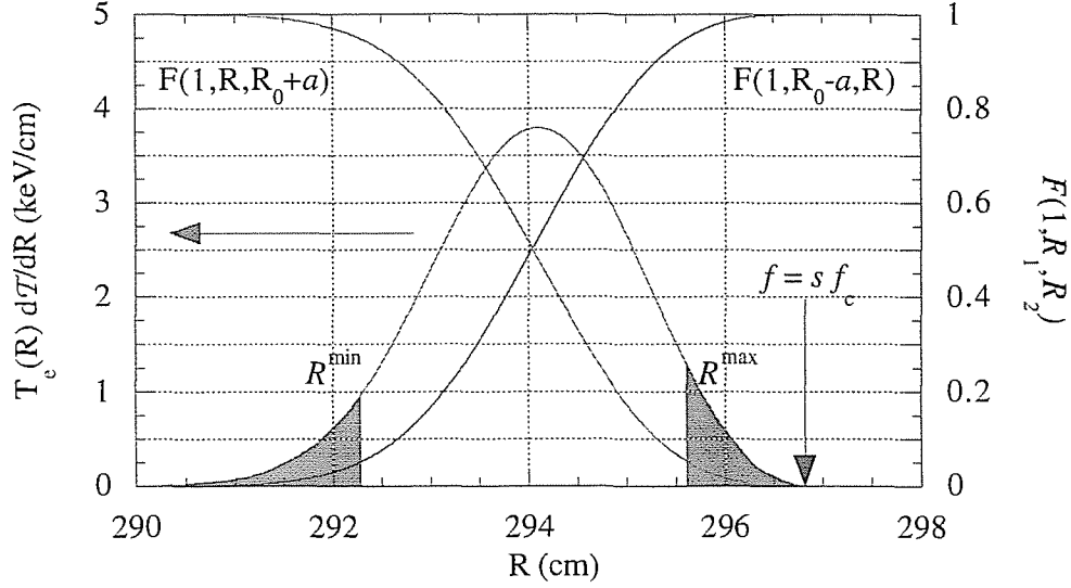
Figure 8: Integrand of Eq. 5 and the function F defined in Eq. 6, along with the values R^{\min} and R^{\max} for g = 0.9 . The shadowed area corresponds to 10 % of the total emission.
