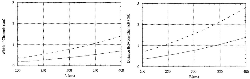
Figure 16: For the heterodyne radiometer (KK3), spatial width (on the left) due to the 250 MHz IF bandwidth of the filters, and distance between consecutive channels, separated 500 MHz, versus the radial position.
