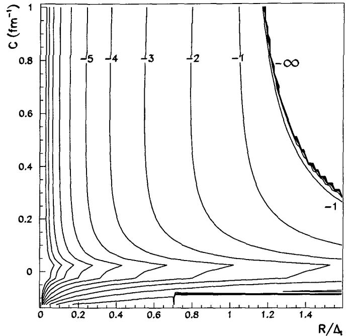
Fig. 5. Same as Fig. 4 for the \log_{10}(B_{CC}/\mu) diagonal element of the inertia tensor. The dimension of B_{CC}/\mu is \text{fm}^{-4} . \mu = A_1 A_2 / A_0 is the reduced mass of the system. The difference between two contour level values is 1.
