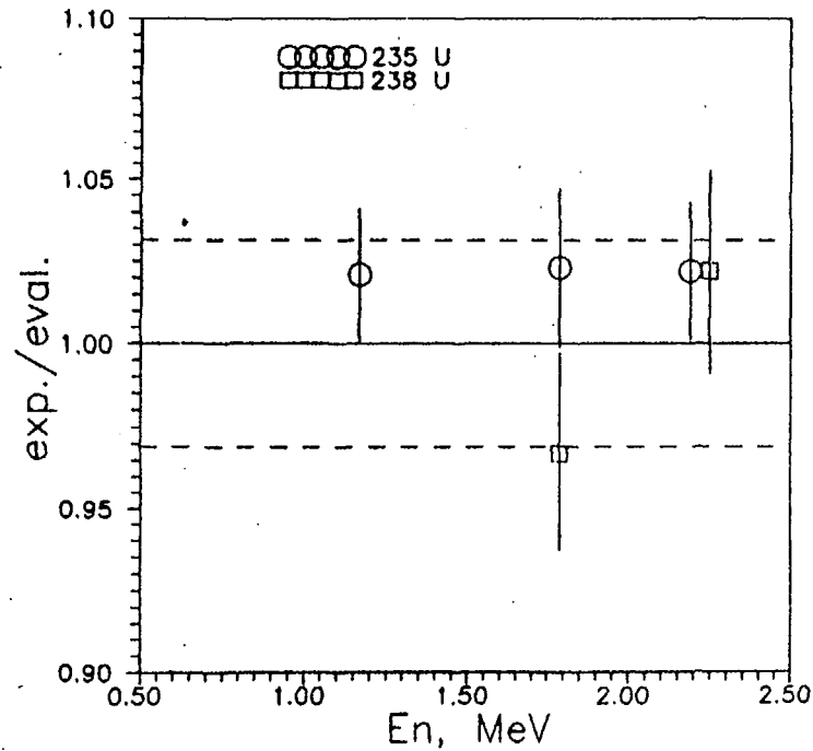
Fig. 7. Relationship of the experimental values of (\nu\sigma_f) and the calculated values from ENDF/B-6. The errors for the points represent errors in the determination of the normalization coefficient for the fission spectrum. They are determined mainly by statistical accuracy. The dashed line shows the evaluated systematic experimental error of \pm 3.2\% .
