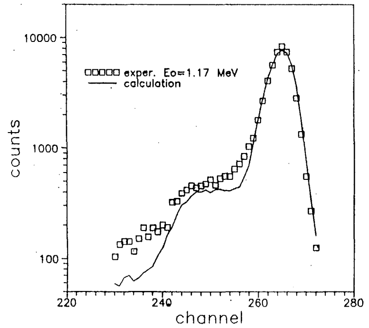
Fig. 2. Time spectrum of neutrons elastically scattered by carbon.
