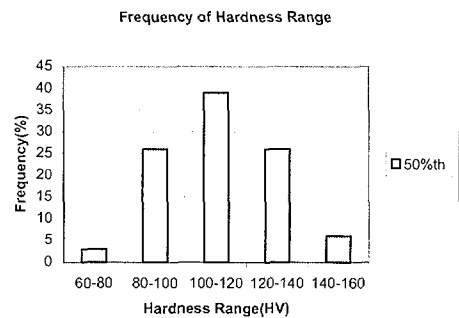
Fig.4. Frequency of hardness range of 50%th dense porous tungsten.
