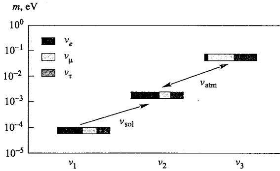
Fig. 1. Neutrino masses and mixings in the scheme with mass hierarchy. Half-tone bars correspond to flavor admixtures in the mass eigenstates \nu_1 , \nu_2 , \nu_3 . The quantity \langle m \rangle is determined by the black bars denoting the admixture of the electron neutrino U_{ei}
