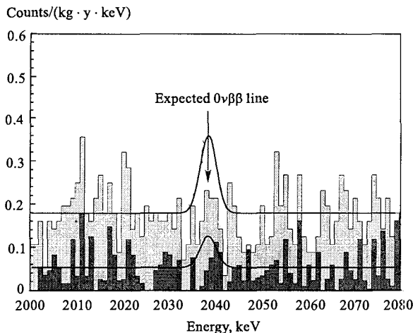
Fig. 6. HEIDELBERG-MOSCOW experiment: energy spectrum in the range between 2000 and 2080 keV, where the peak from neutrinoless double beta decay is expected. The open histogram denotes the overall sum spectrum without PSA after 55.9 kg·y of measurement (since 1992). The filled histogram corresponds to the SSE data after 37.2 kg·y. Also shown are the excluded (90% C.L.) peak areas from the two spectra
