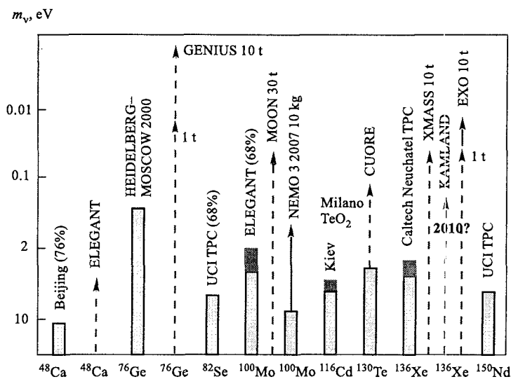
Fig. 5. Present situation, 2000, and expectation for the future of the most promising \beta\beta experiments. Light parts of the bars — present status; dark parts — expectation for running experiments; solid and dashed lines — experiments under construction and proposed experiments. For references see [3,39,65]
