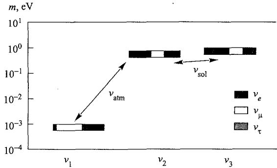
Fig. 3. Neutrino masses and mixing in the inverse hierarchy scenario
