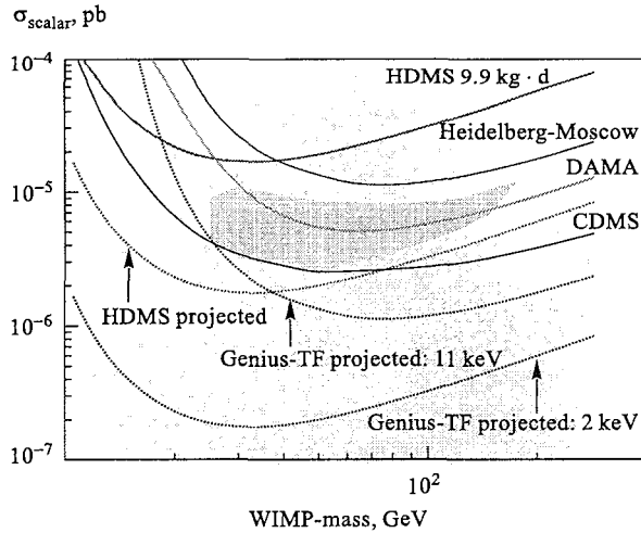
Fig. 15. WIMP-nucleon cross section limits as a function of the WIMP mass for spin-independent interactions. The solid lines are current limits of the HEIDELBERG–MOSCOW experiment [8], the HDMS prototype [9], the DAMA experiment [70] and the CDMS experiment [72]. The dashed curves are the expectation for HDMS [9] and for GENIUS-TF with an energy threshold of 11 and 2 keV respectively, and a background index of 2 events/(kg·y·keV) below 50 keV. The filled contour represents the 2\sigma evidence region of the DAMA experiment [71]. The experimental limits are compared to expectations (scatter plot) for WIMP-neutralinos calculated in the MSSM parameter space under the assumption that all superpartner masses are lower than 300–400 GeV [33] (from [40,41]).
