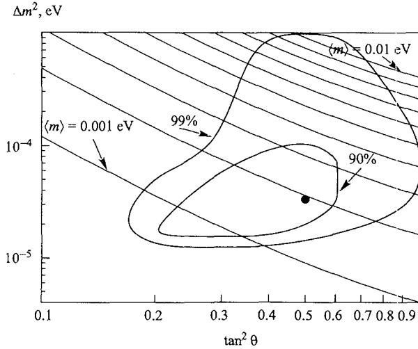
Fig. 2. Double beta decay observable \langle m \rangle and oscillation parameters in the case of the MSW large mixing angle solution of the solar neutrino deficit, where the dominant contribution to \langle m \rangle comes from the second state. Shown are lines of constant \langle m \rangle , the lowest line corresponding to \langle m_\nu \rangle = 0.001 \text{ eV} , the upper line to 0.01 \text{ eV} . The inner and outer closed lines show the regions allowed by present solar neutrino experiments with 90% C.L. and 99% C.L., respectively. Double beta decay with sufficient sensitivity could check the LMA MSW solution. Complementary information could be obtained from the search for a day-night effect and spectral distortions in future solar neutrino experiments as well as a disappearance signal in KAMLAND
