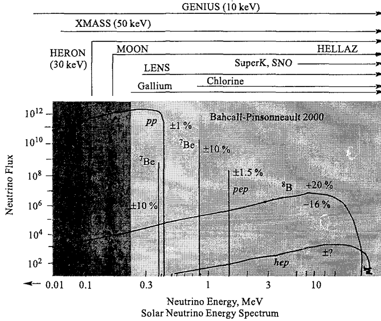
Fig. 12. The sensitivity (thresholds) of different running and projected solar neutrino detectors (see [68] and HEIDELBERG-MOSCOW home-page: http://www.mpi-hd.mpg.de/non_acc/ )
