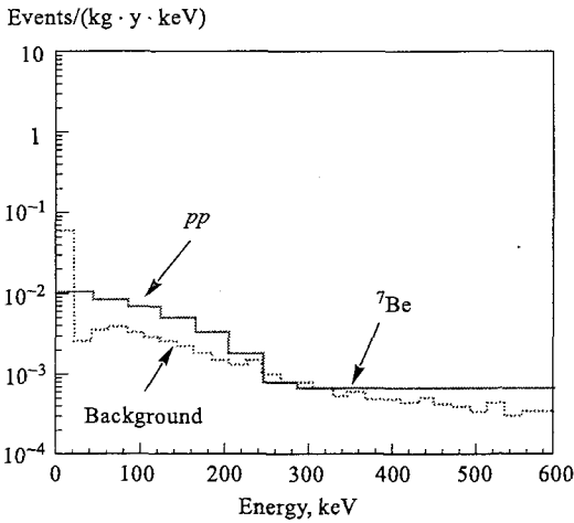
Fig. 13. Simulated spectrum of low-energy solar neutrinos (according to SSM) for the GENIUS detector (1 tonne of natural or enriched Ge) (from [6])
