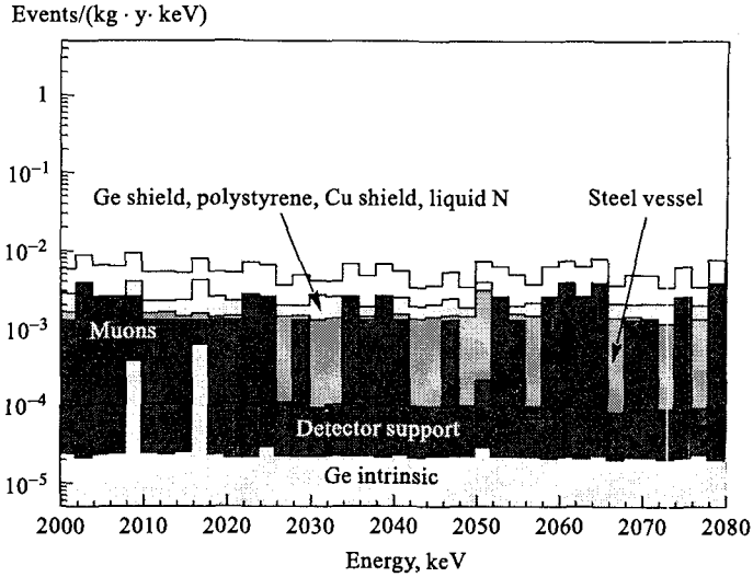
Fig. 16. Simulated spectra of the dominant background sources for the enriched ^{76}\text{Ge} detectors of the HEIDELBERG–MOSCOW experiment in the GENIUS-TF setup. The energy region relevant for the search of the neutrinoless double beta decay is shown. The upper solid line represents the sum spectrum of all the simulated components (from [40,41])
