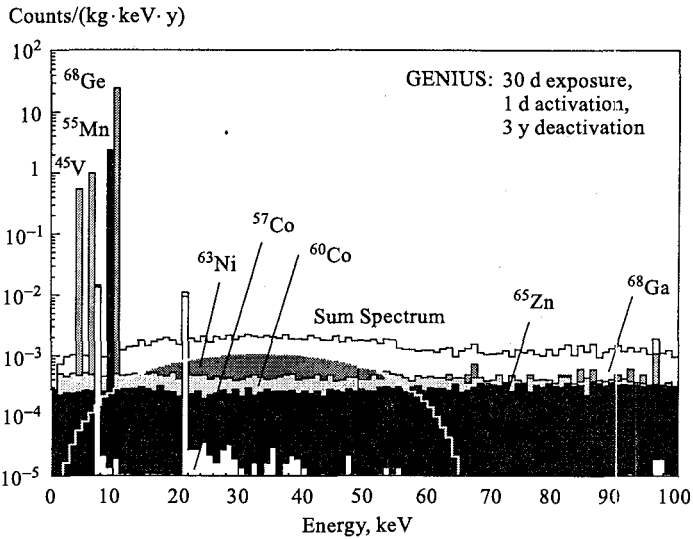
Fig. 10. Simulated cosmogenic background during detector production. Assumptions: 30-day exposure of material before processing, 1-day activation after zone refining, 3-year deactivation underground (see [7,39])
