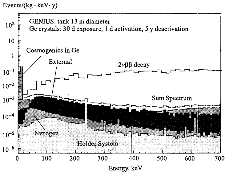
Fig. 11. Total background in a 13 m liquid nitrogen tank for detectors produced as described in Fig. 10 (see [7,39])
