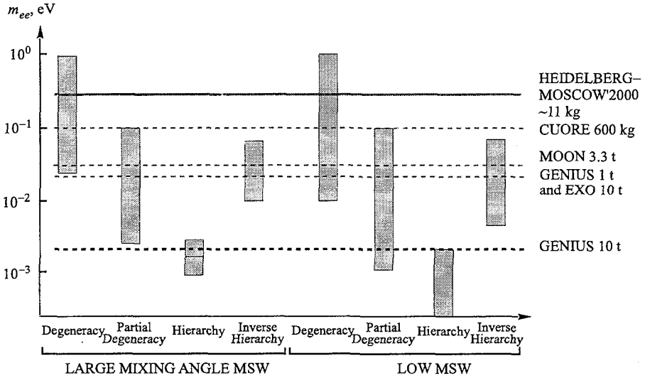
Fig. 4. Summary of values for m_{ee} = \langle m \rangle expected from neutrino oscillation experiments (status NEUTRINO'2000), in the different schemes discussed in this paper. For a more general analysis see [1]. The expectations are compared with the recent neutrino mass limits obtained from the HEIDELBERG-MOSCOW experiment [7,19], as well as the expected sensitivities for the CUORE [50], MOON [47], EXO [48] proposals and the 1 tonne and 10 tonne proposal of GENIUS [12,13]
