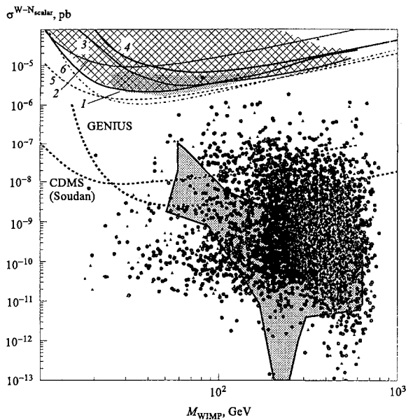
Fig. 8. WIMP-nucleon cross section limits in pb for scalar interactions as function of the WIMP mass in GeV. Shown are contour lines of present experimental limits (solid lines: 1 — CDMS, 2 — HDMS prototype, 3 — DAMA NAT, 4 — HEIDELBERG–MOSCOW ^{76}\text{Ge} ) and of projected experiments (dashed lines: 5 — HDMS projection, 6 — GENIUS-TF projection — 4 keV threshold with NAT2). Also presented is the region of evidence published by DAMA. The theoretical expectations are shown by a scatter plot (from [32]) and by grey region (from [38]). Only GENIUS will be able to probe the shown range also by the signature from seasonal modulations
