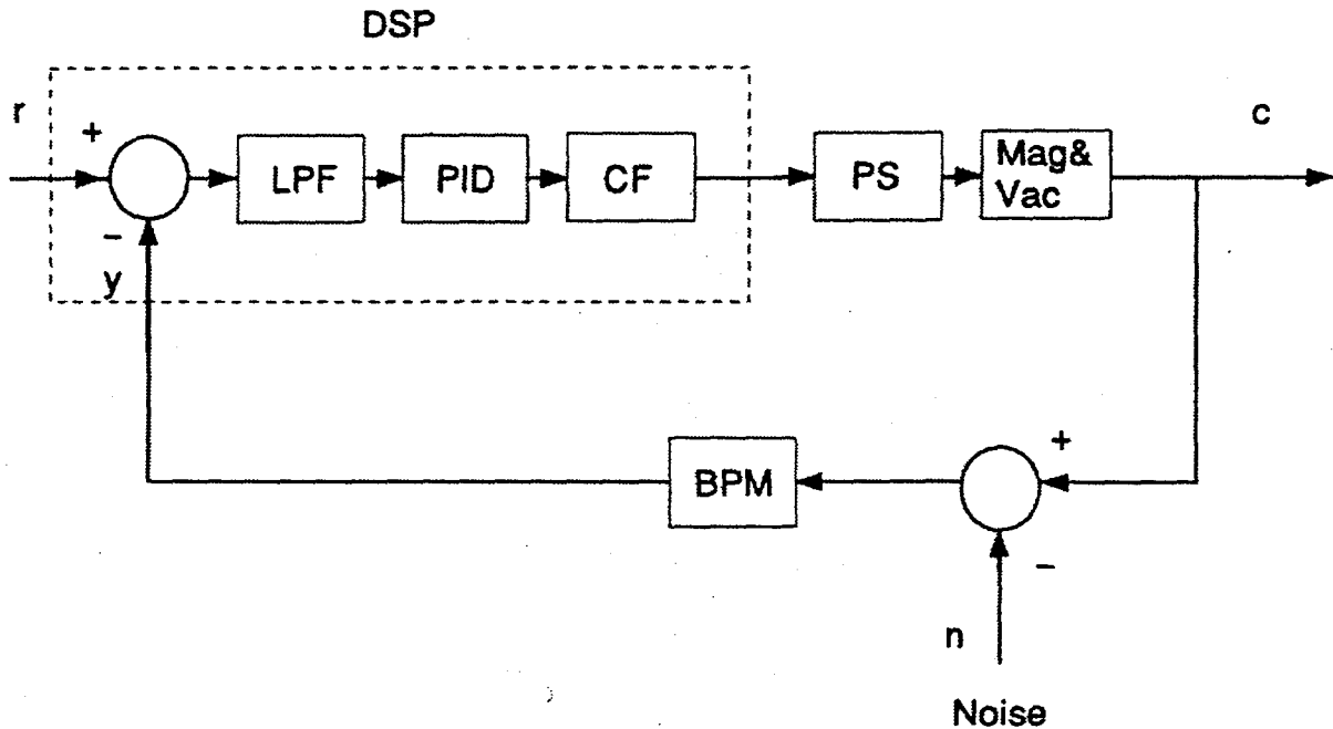
Fig. 3. Block diagram of the actual closed loop system of the global orbit control
