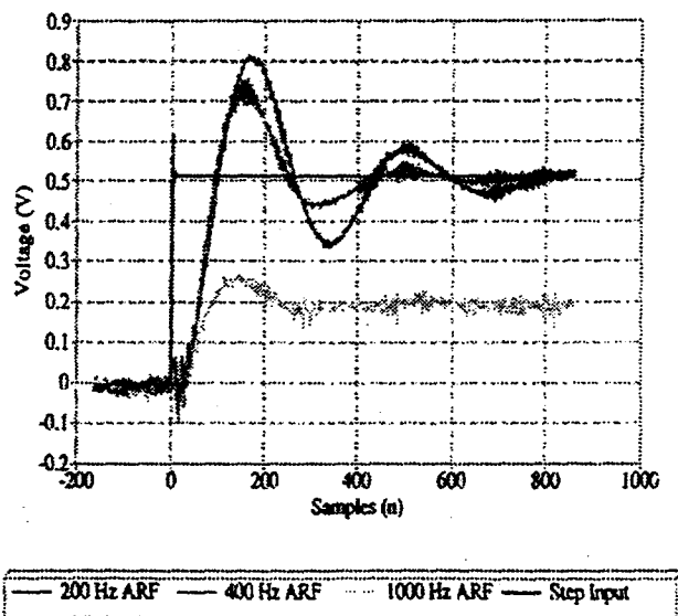
Step response of K_p = 2.5 , K_i = 0.25 , and K_d = 0 .
