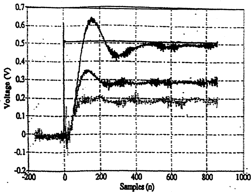
Figure 9 Step response of K_p = 4 , K_i = 0.05 , and K_d = 0 .
