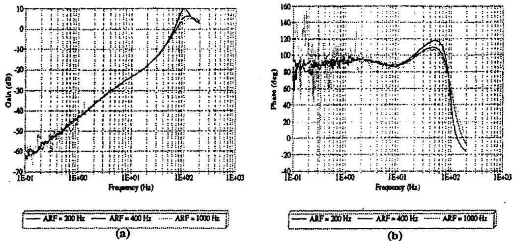
Frequency response of the noise transfer function with K_p=2.5 , K_i=0.25 , and K_d=0 .
