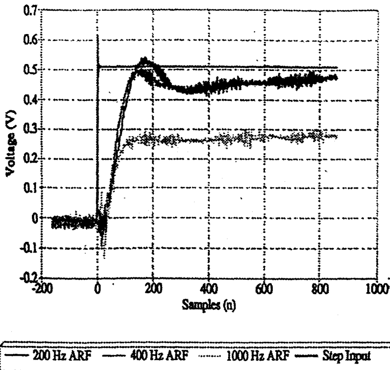
Figure 8 Step response of K_p = 2.5 , K_i = 0.05 , and K_d = 0 .
