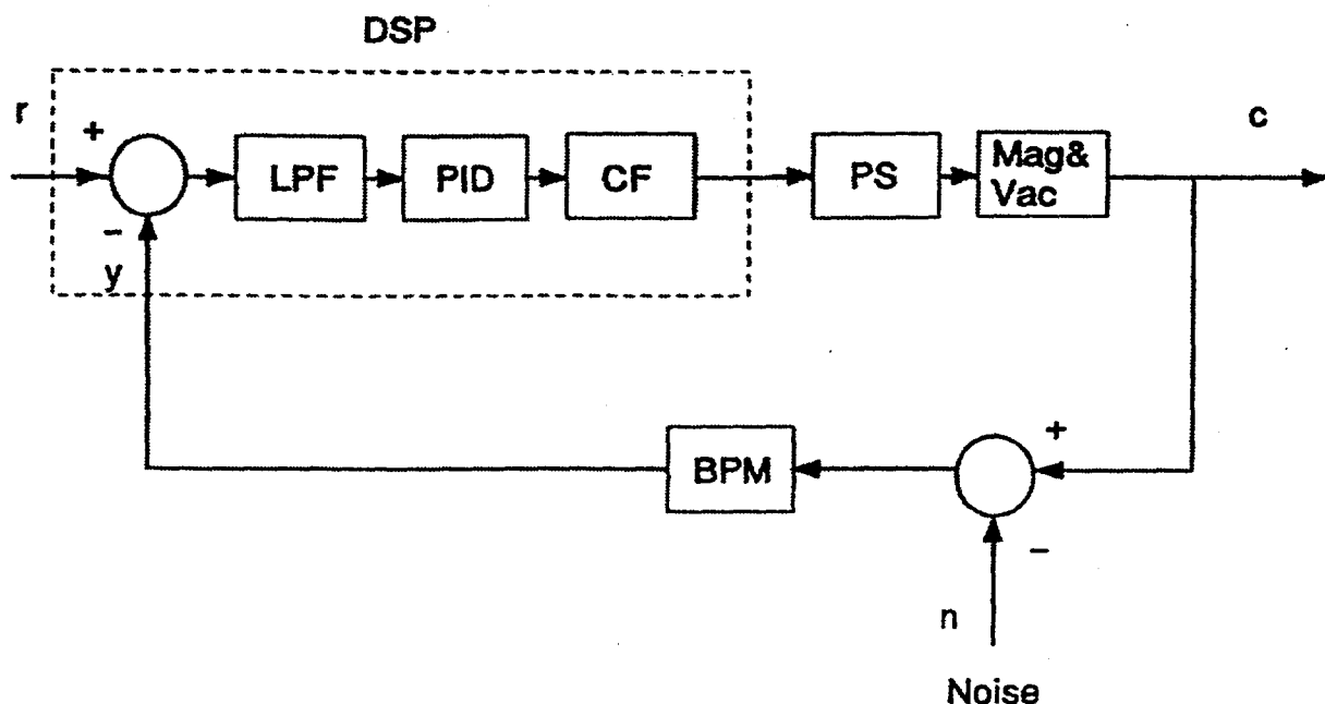
Fig. 1. Simplified block diagram of the APS diagnostic closed loop feedback system
