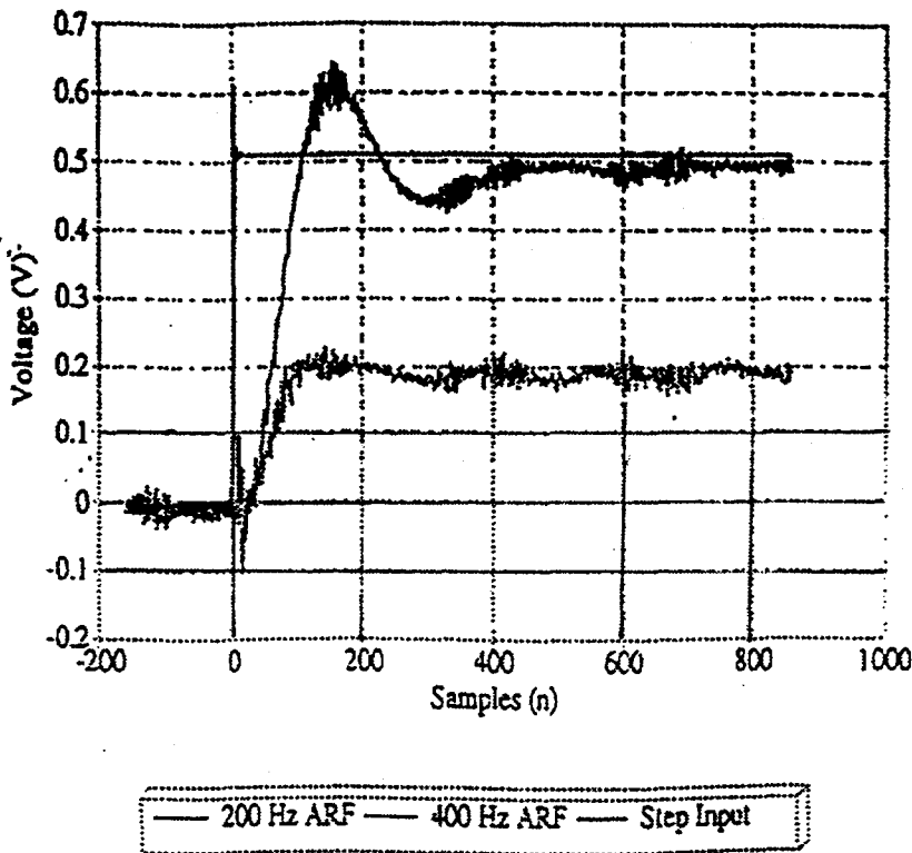
Figure 11 Step response of K_p = 3 , K_i = 0.1 , and K_d = 1 .
