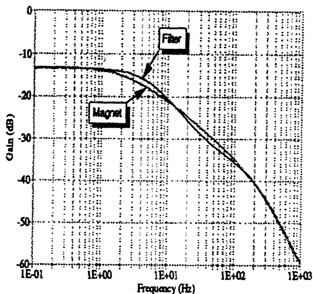
Fig. 5. Frequency response of the digital filter and the actual magnet and vacuum chamber
