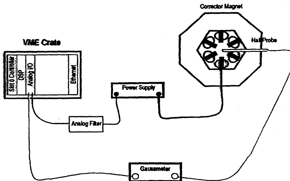
Fig. 4. DSP global orbit feedback test setup
