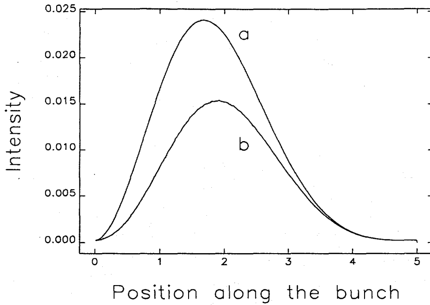
Fig. 1. Coherent SASE intensity |a_{coh}|^2 versus 2\rho\theta for a flat-top bunch (a) without initial energy spread, (b) with a flat-top energy spread of width \rho , at \bar{z} = 5 .
