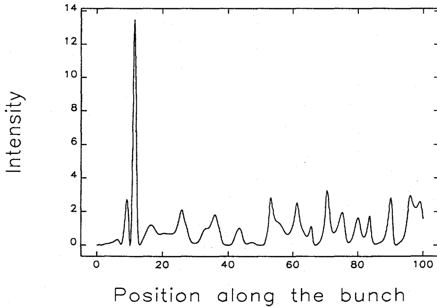
Fig. 2. Coherent and incoherent SASE intensity |a|^2 vs. 2\rho\theta for a flat-top bunch ( 0 < 2\rho\theta < 100 ) without initial energy spread at \bar{z} = 15 .
