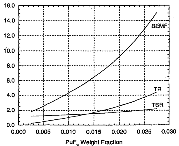
Fig. 1. Blanket energy multiplication factor (BEMF), transmutation rate (TR - kg/MW.y), and tritium breeding ratio (TBR) as function of the PuF 3 weight fraction in the Flibe molten salt.
