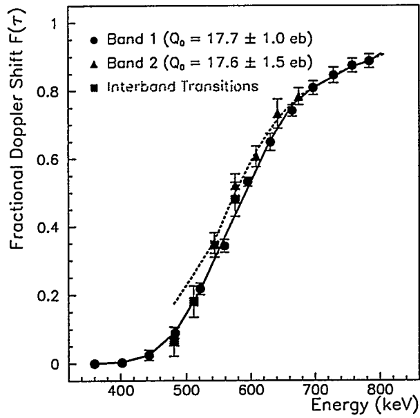
Figure 1.1 Measured fractional shifts F(\tau) for \gamma -rays in the two SD bands (1 and 2) and for the inter-band transitions in ^{190}\text{Hg} . The F(\tau) values for the linking transitions are plotted at the \gamma -ray energies of the corresponding in-band transitions of band 2. The solid and dashed curves represent the best fits corresponding to the values of the Q_0 moment given in the figure.
