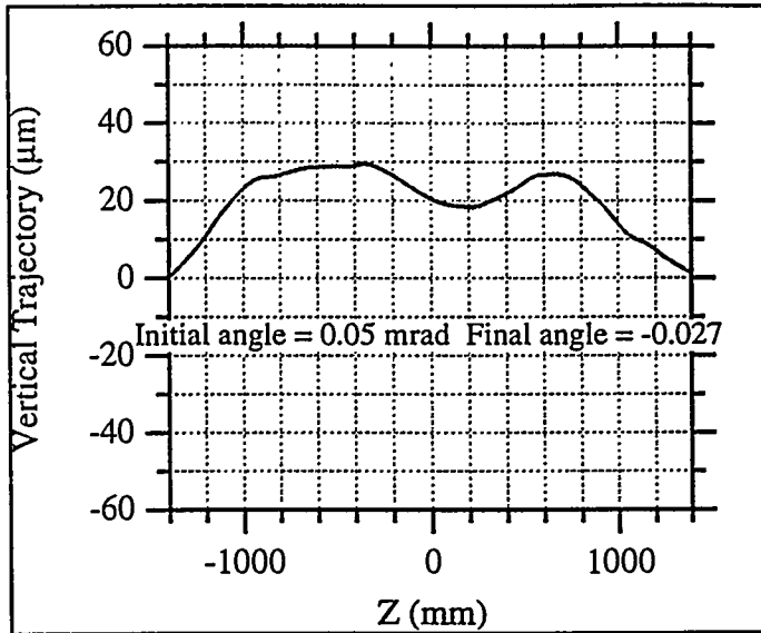
Fig. 3 Vertical Trajectory of the First Two FEL Devices
