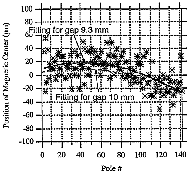
Fig. 4. Position of magnetic centers for UNA#21. The solid line shows the fit to the data; the corresponding fit for a gap of 10.0 mm is shown for reference. The overall 40 \mu\text{m} slope is due to the geometrical misalignment of the sensor and device.
