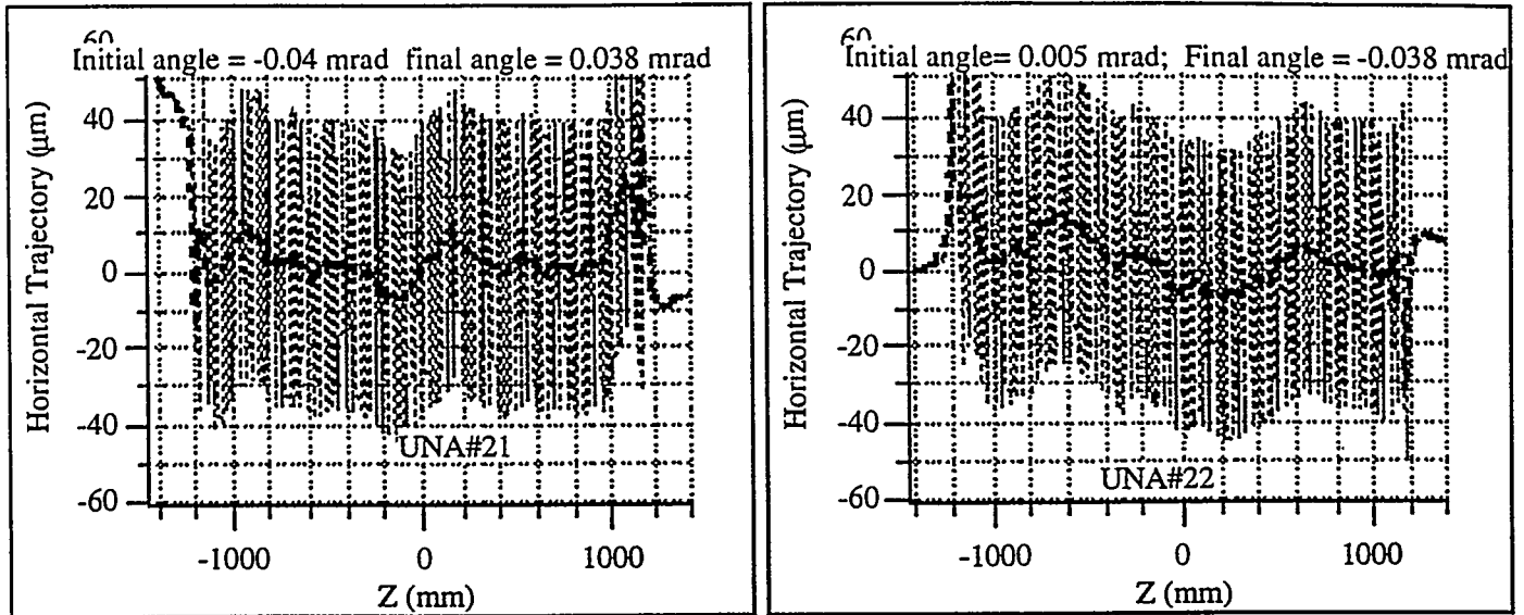
Fig. 2 Horizontal trajectory of the first two FEL devices. The dark line is the wiggle-averaged trajectory.
