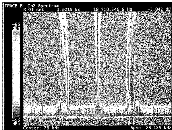
Figure 7 – Spectrum from acceleration ramp showing a revolution line (center), and betatron sidebands to either side. Beginning of ramp is at top, broadband green blending into yellow at bottom is noise due to beam loss at transition. Tunes are coupled so that both horizontal and vertical show up in this vertical spectrum. Lines also appear at .25 and .375 with increased losses, suggesting beam in islands.
