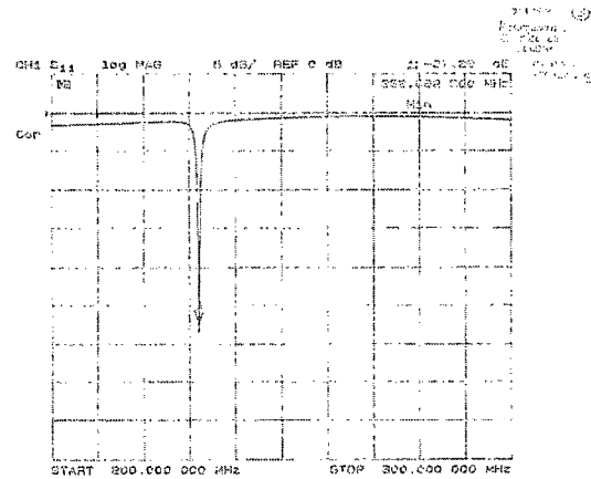
Figure 6 - Reflection coefficient for the Horizontal Plane Hybrid Difference port, Movable BPM located at 2 O'clock on the Yellow beam line
