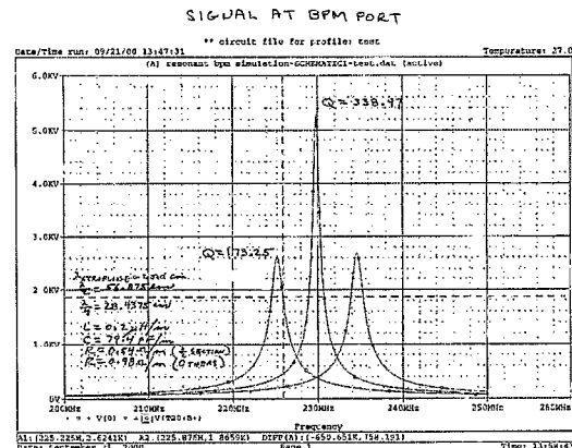
Figure 4 – Simulated Signal at BPM Port. Response to difference mode signal of unit value. Note; unloaded Q at resonance is twice loaded Q with shifted resonant response.
