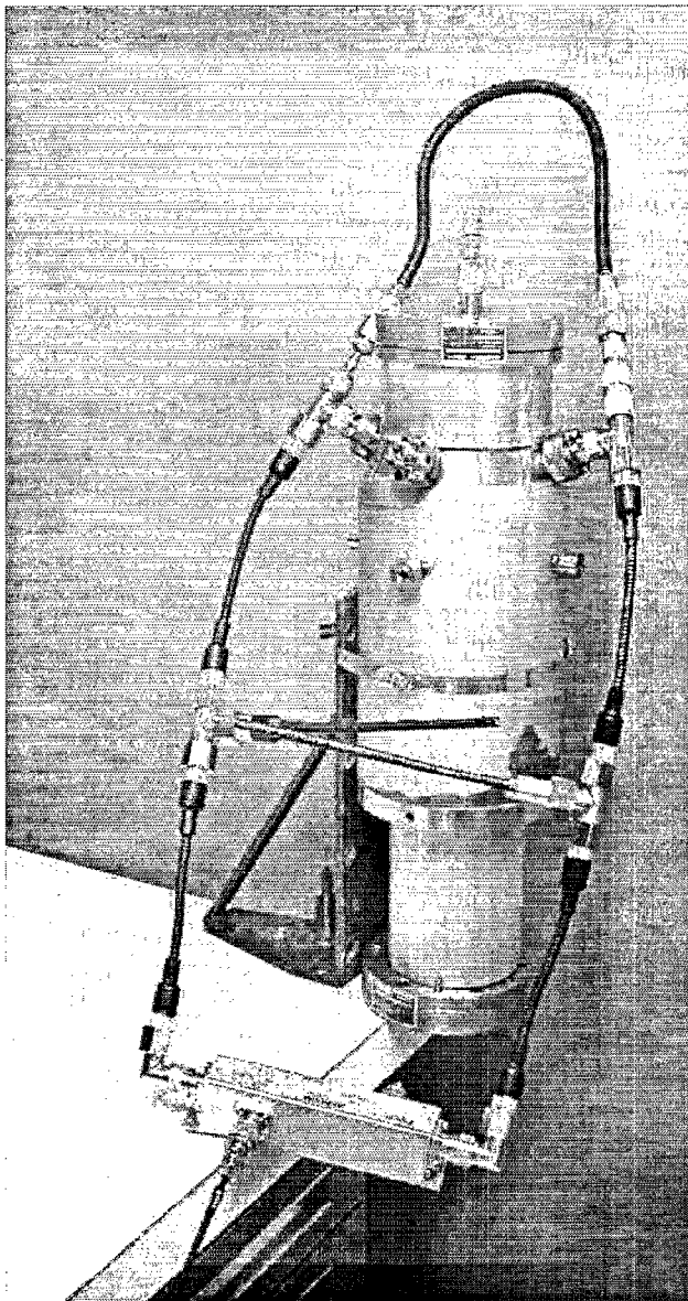
Figure 5 – Photo of stub tuned resonant BPM showing testing configuration. Matching sections at each end carry a RF signal through a center conductor to a termination. Output is taken from the difference port of a Hybrid transformer.
