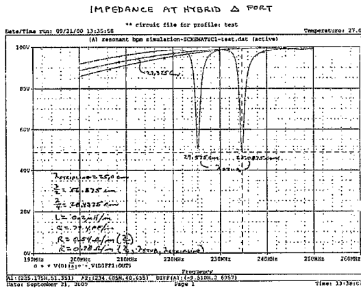
Figure 2 – Simulation of Impedance at Hybrid Difference Port. Note; poor match with stub cut to exactly quarter wave.
