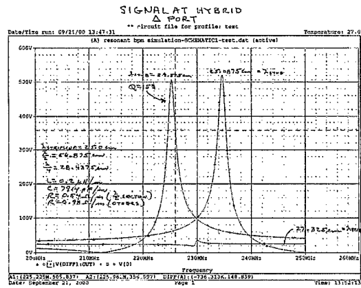
Figure 3 – Simulated Signal at Hybrid Difference Port. Response to difference mode signal of unit value. Note; very little response with stub cut to exactly quarter wave.
