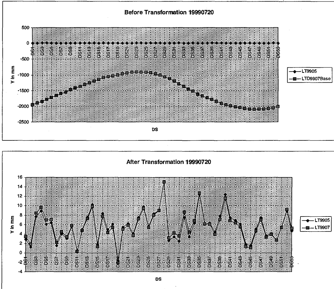
Fig 12. Heights of Floor reference before and after transformation in July 1999
