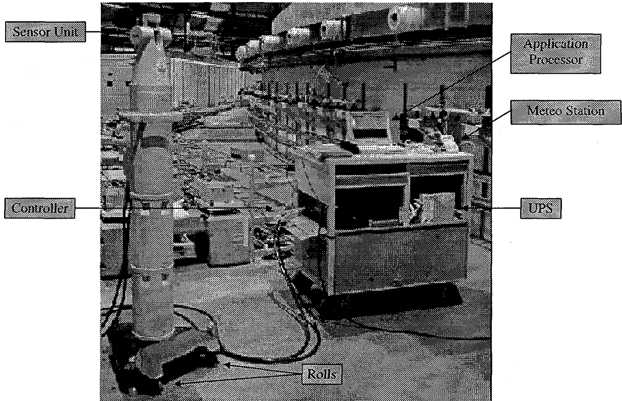
Fig. 5 LTD500 In the SLS tunnel
