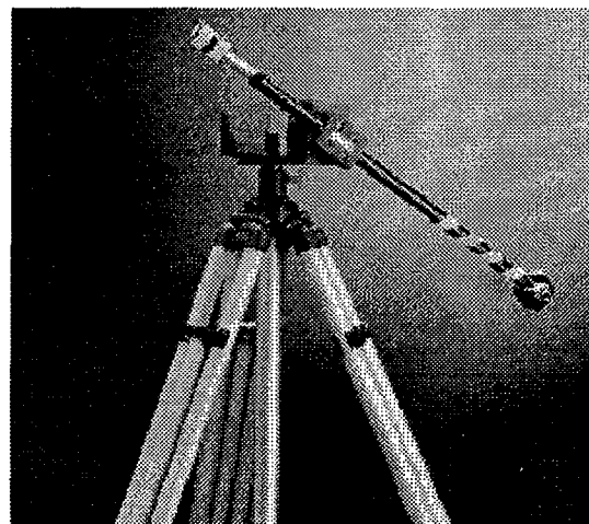
Fig. 7 Mount ball bar
