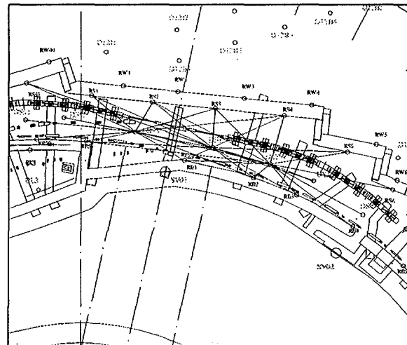
Fig. 10. LTD500 measurement in tunnel
