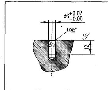
Fig. 14 Reference hole
