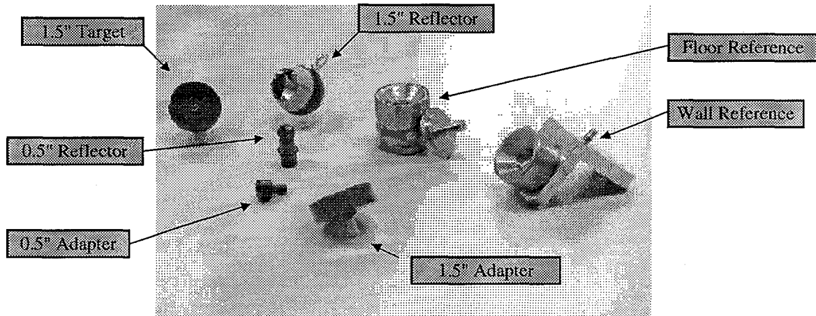
Fig. 4 References, reflectors and adapters
