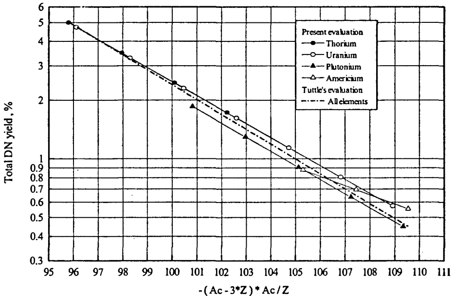
Fig.6. Dependence of the total DN yields on parameter P = -(A_c - 3Z) \cdot A_c / Z .
