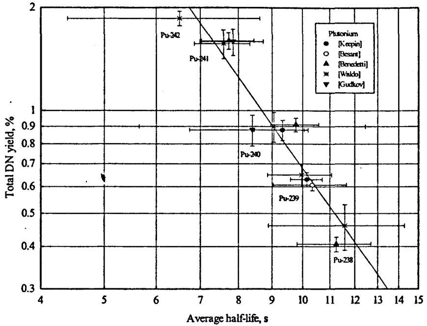
Fig.4. Total DN yield as a function of average half life of DN precursors for Pu
