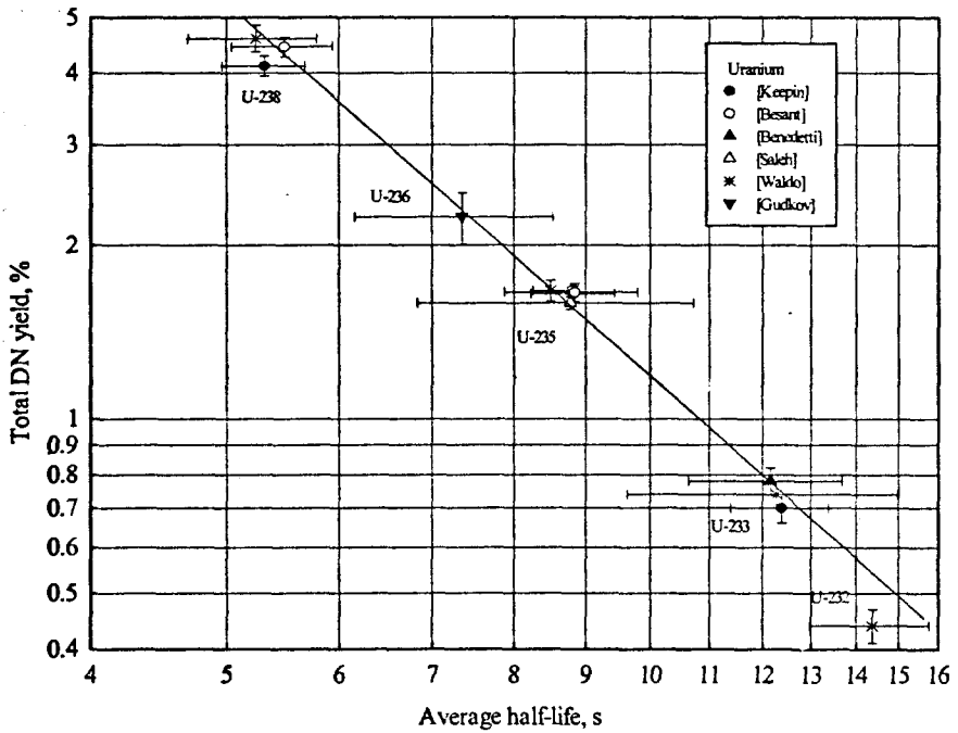
Fig.3. Total DN yield as a function of average half life of DN precursors for U
