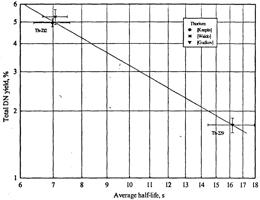
Fig.2. Total DN yield as a function of average half life of DN precursors for Th
