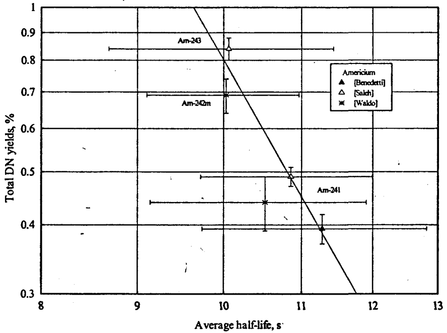
Fig.5. Total DN yield as a function of average half life of DN precursors for Am
