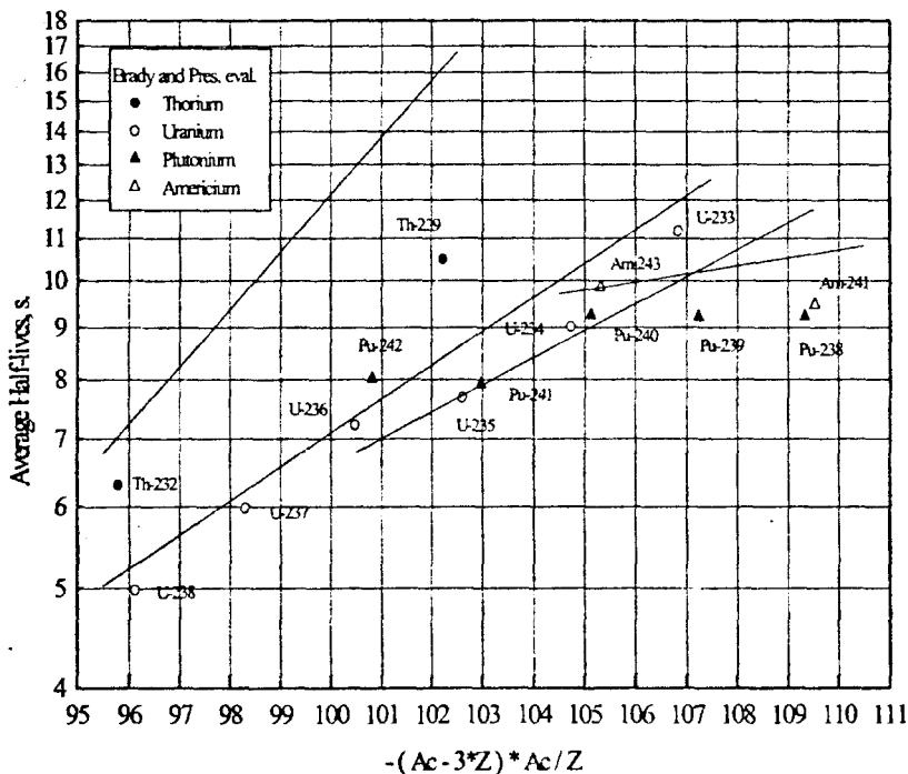
Fig. 7. Dependence of the average half life of DN precursors on parameter -(A_c-3Z)A_c/Z . Solid lines - present systematics (see Fig.1), points - the ENDF/B-VI data
