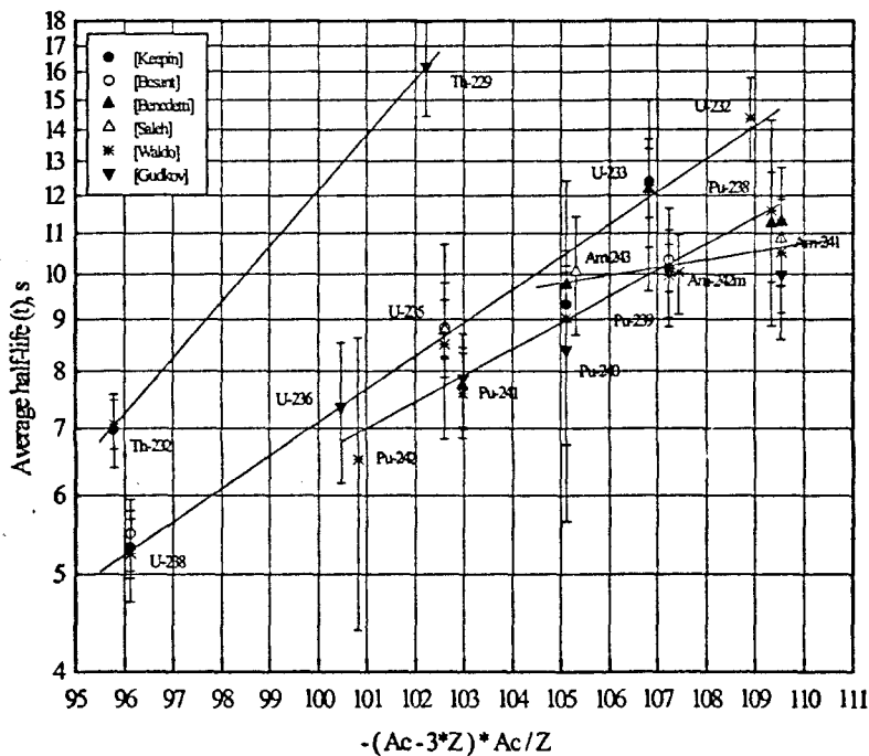
Fig.1. Systematics of the average half life of DN precursors for Th, U, Pu, Am elements
