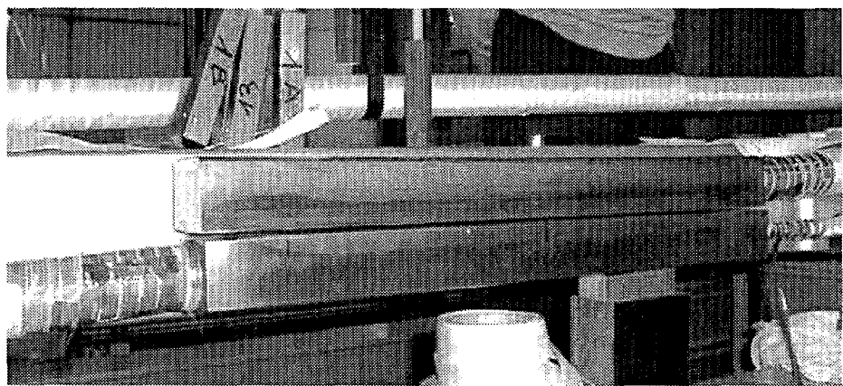
Fig. 5b: Two adjacent terminations of a DP module inner joint before being soldered and clamped together
