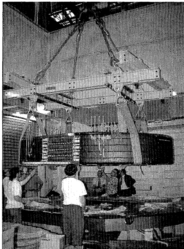
Fig. 4: The impregnated winding pack consisting of five double-pancake modules
