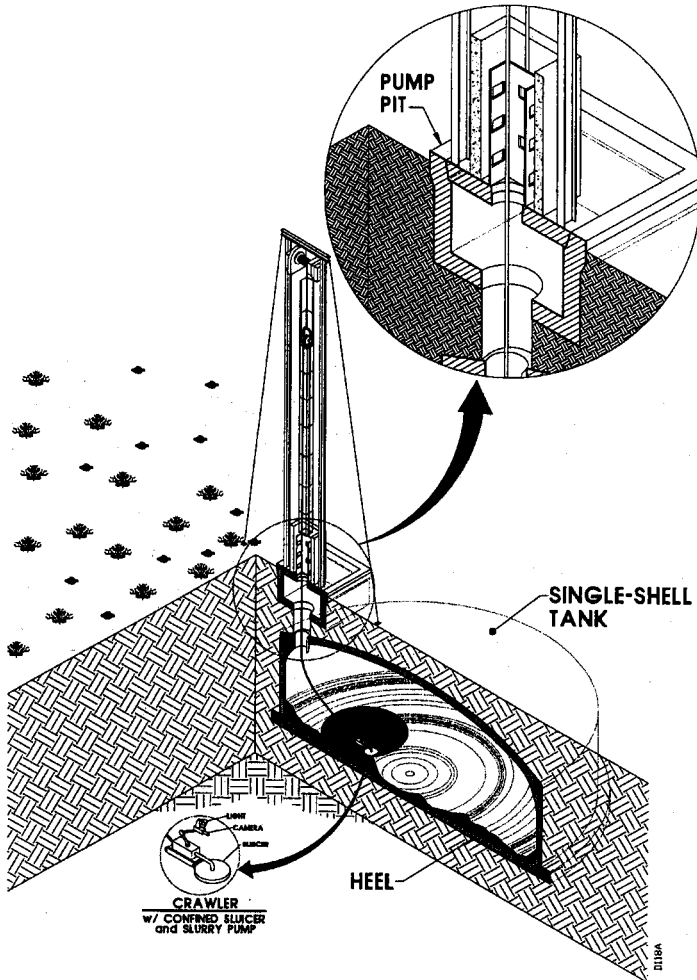
Figure 1. Vehicle-Based Waste Retrieval System.
