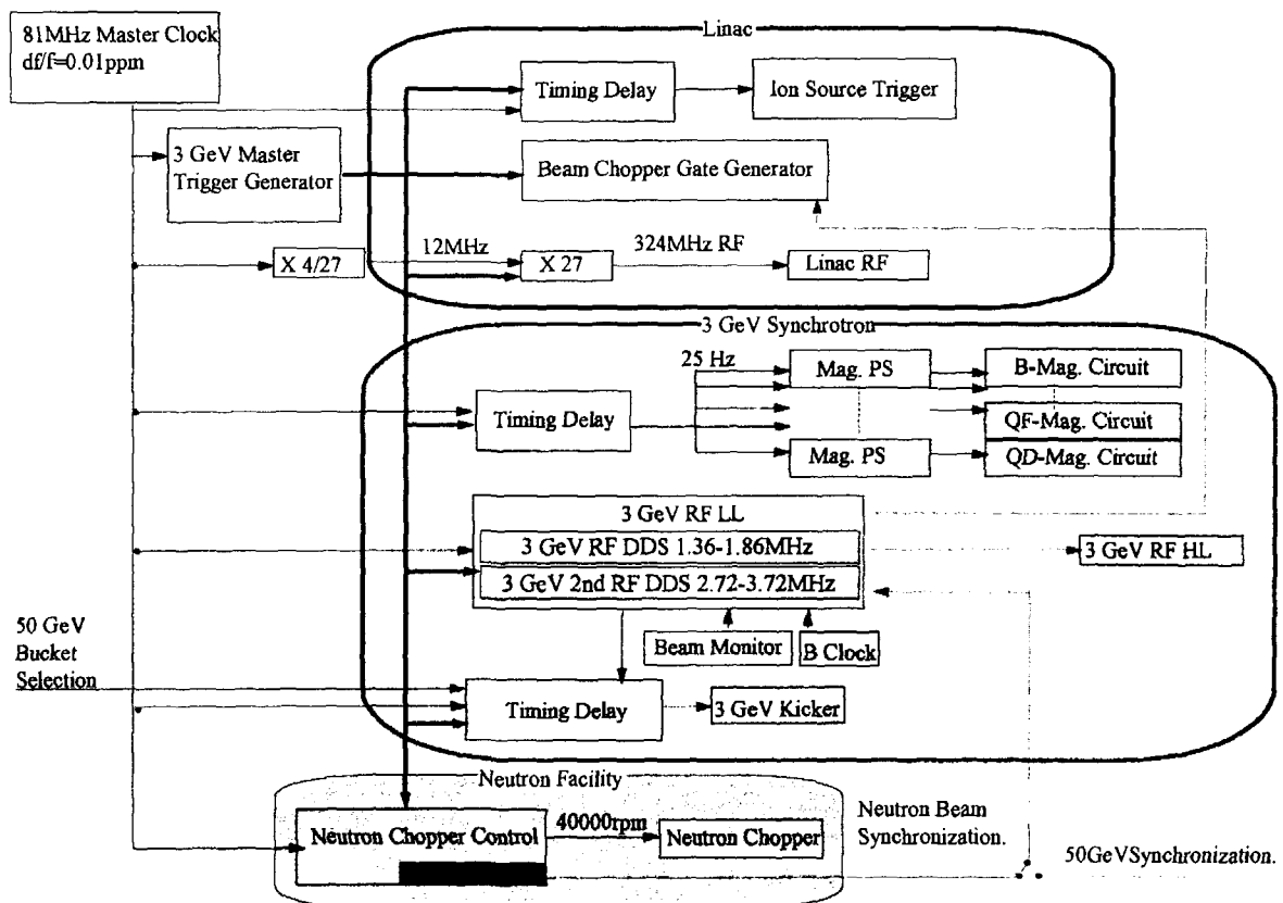
Figure 1. The block diagram of the 3 GeV timing control.
