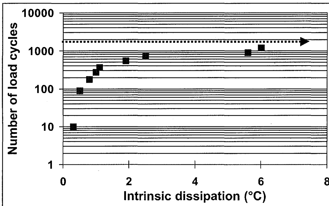
Figure 2. Fatigue lifetime evaluation of a column base of the reinforced concrete structure subject to seismic type loading.
