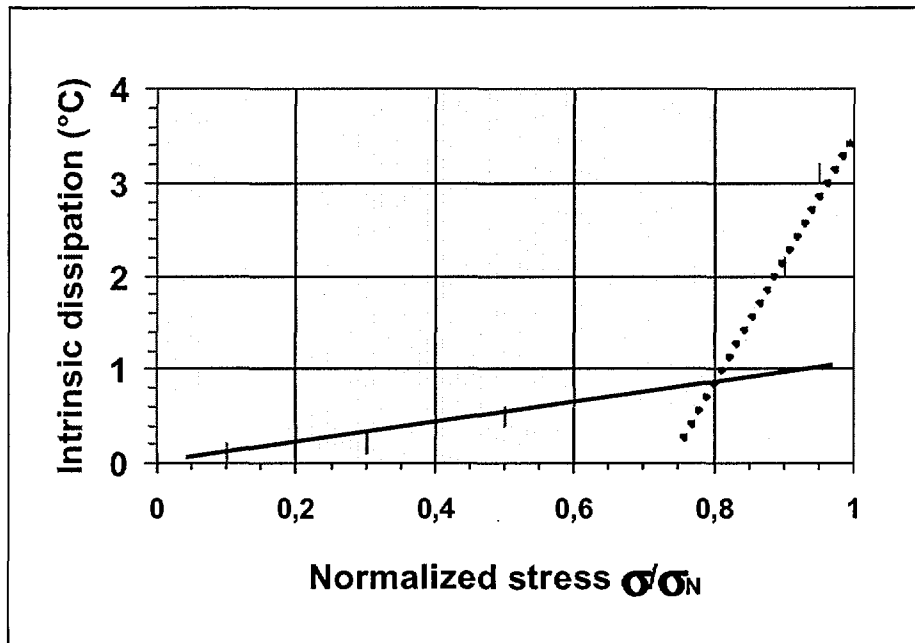
Figure 1. The fatigue limit (FL) of the concrete specimen under compressive loading is graphically determined by a drastic change of the dissipative regime.
