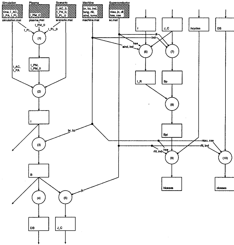
Figure 4: Dataflow.
