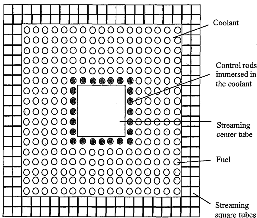
Figure 1. Schematic of Hejzlar streaming assembly.
