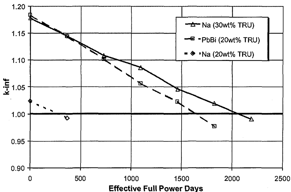
Figure 3. Reactivity comparison at 86 W/cm.
