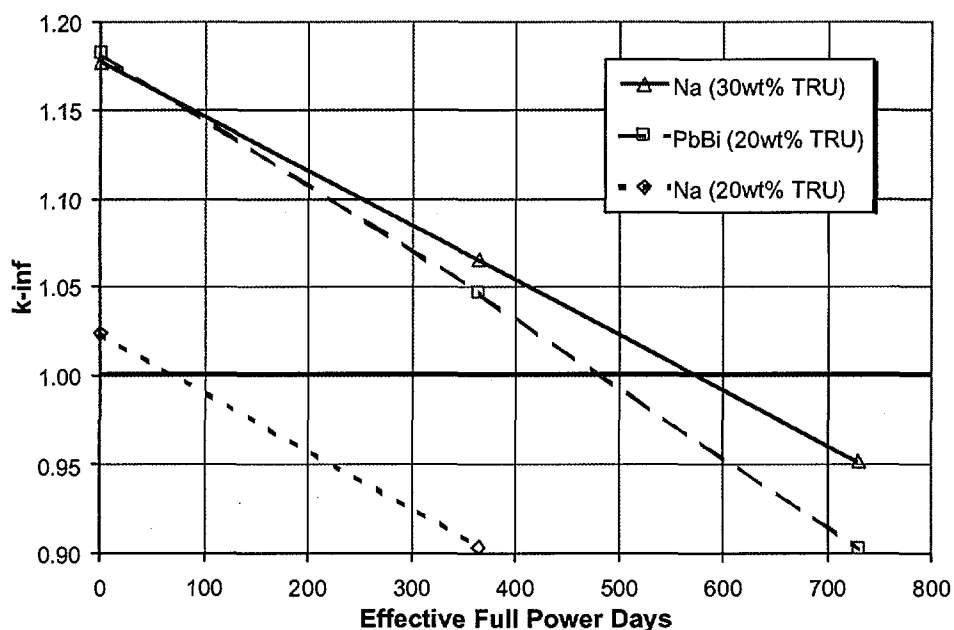
Figure 2. Reactivity comparison at 367.5 W/cm.
