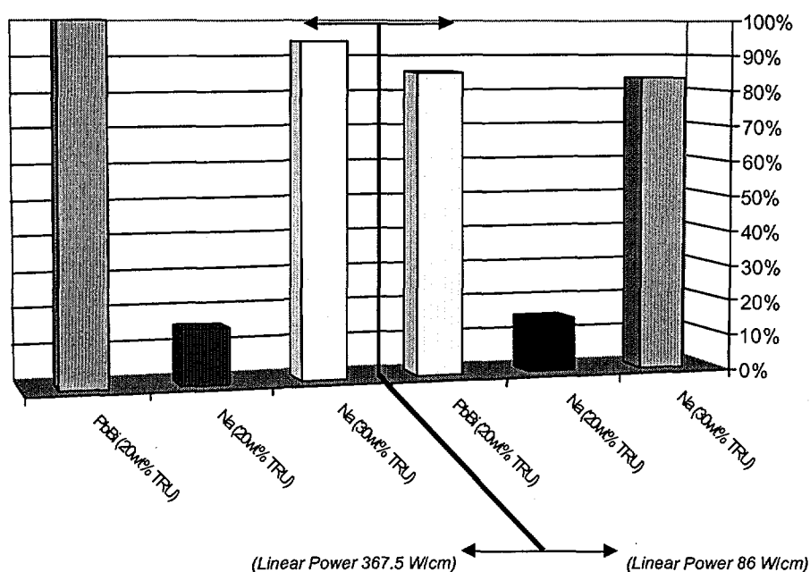
Figure 6. Normalized 1-batch core actinide burnup comparison.
