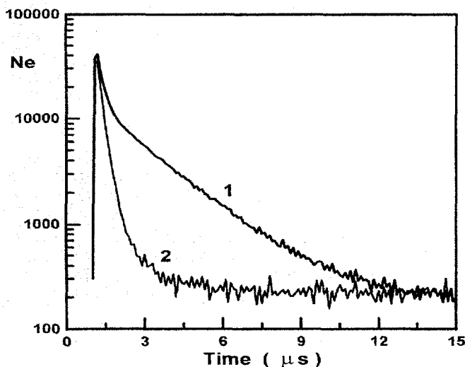
Fig. 5. Electron decay time spectrum: 1) target filled with deuterium; 2) empty target
