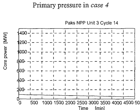
Fig. 5. Core power history in case 4
