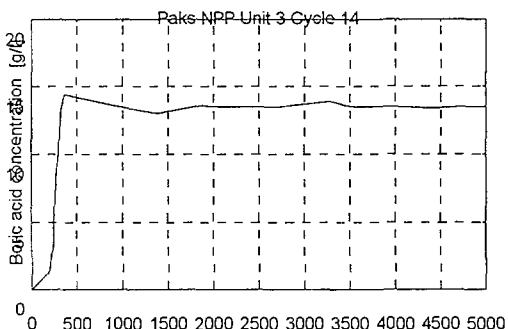
Fig. 3. Boric acid concentration in case 4
