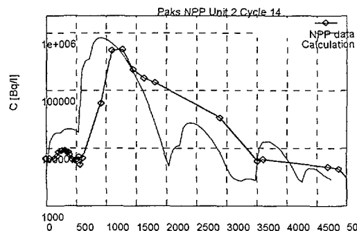
Fig. 6. Measured and calculated ^{131}\text{I} activity concentration during shutdown period, case 1
