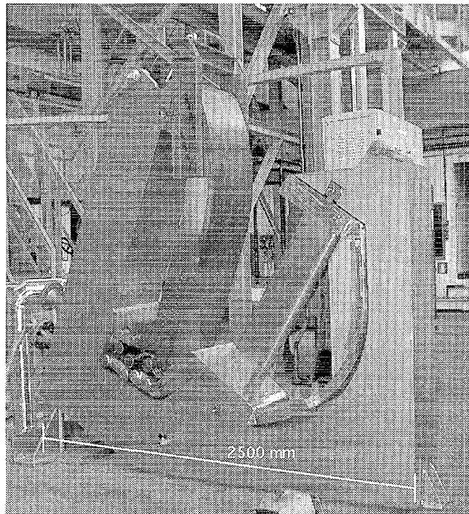
Outboard Cassette Body with integration prototypes assembled onto it
