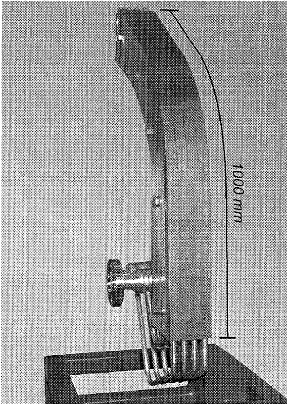
Vertical Target prototype with CFC and tungsten armour
