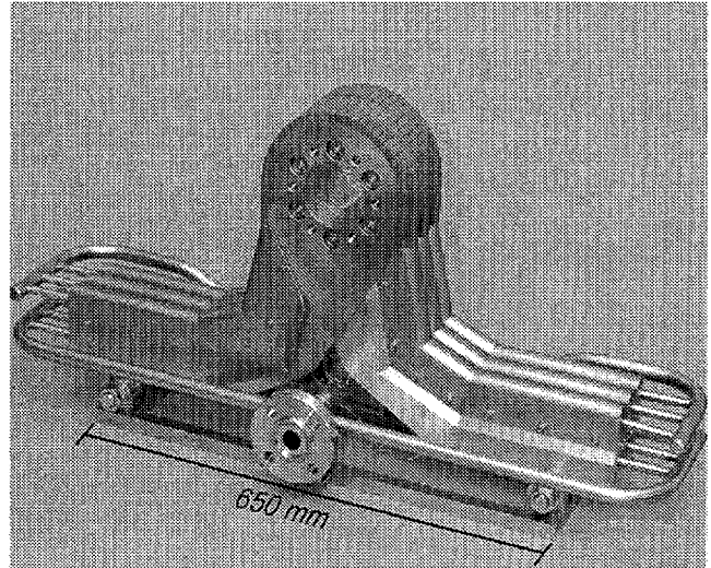
Dome Liner prototype with tungsten armour
