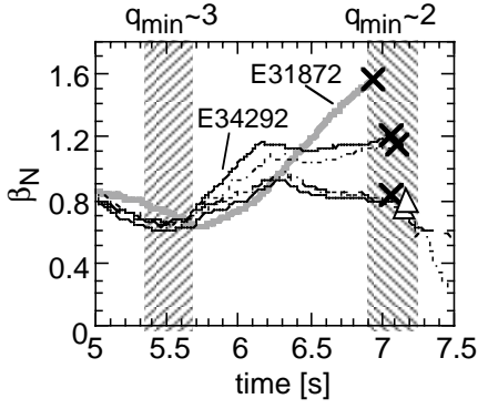
FIG. 1. Evolution of \beta_N in high I_p reversed shear plasmas ( B_t \sim 4.35 T, I_p = 2.4 - 2.6 MA). Crosses denote disruptive beta collapses while triangles denote non-disruptive collapses.
