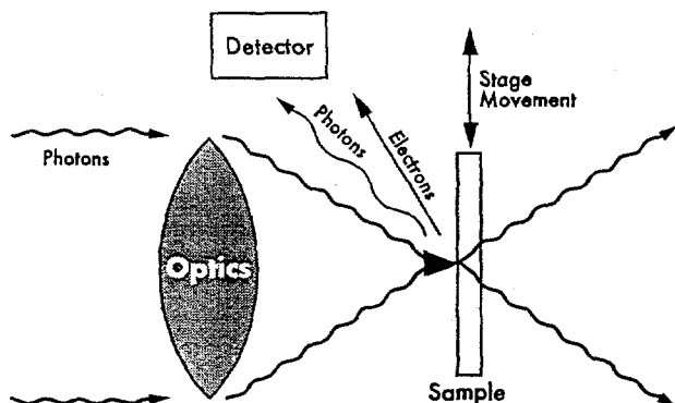
Scanning X-Ray Microscope (~ 50 nm spot)
