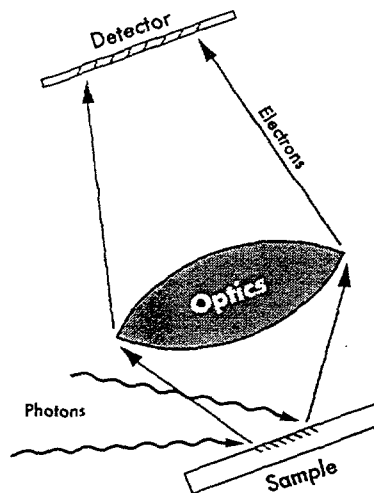
Figure 5. Both scanning and imaging x-ray microscopes can take advantage of high-brightness synchrotron light to produce images at high resolution.
