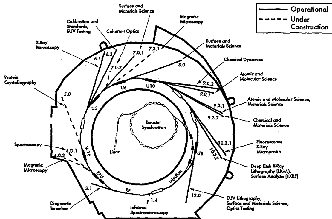
Figure 8. A plan view of the Advanced Light Source and its beamlines shows the wide range of fundamental and applied studies underway at that facility. Others will be developed as new capabilities and new needs arise.
