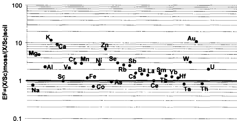
Fig. 6 Enrichment factors of elements in moss with respect to soil
