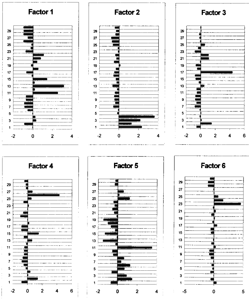
Fig. 2 Plots of factor scores for moss samples
