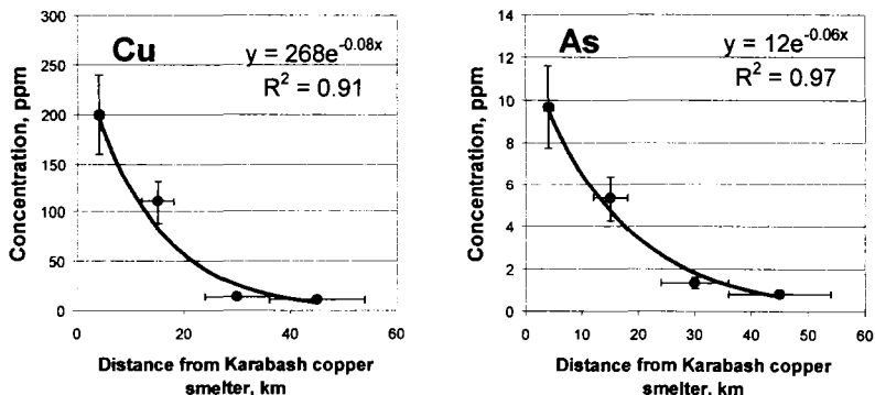
Fig. 4 Gradient of Cu, As (moss samples)
