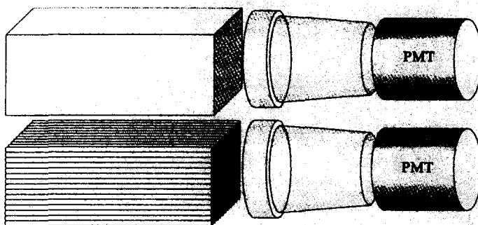
Fig. 2. Detector schemes: original configuration — with bar of scintillator plastic (top), and proposed change — bundle of scintillating fibers (bottom)
