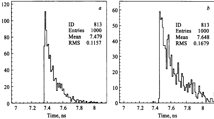
Fig. 3. Distribution of time of photon propagation along the scintillating bar (a) and the bundle of scintillating fibers (b)
