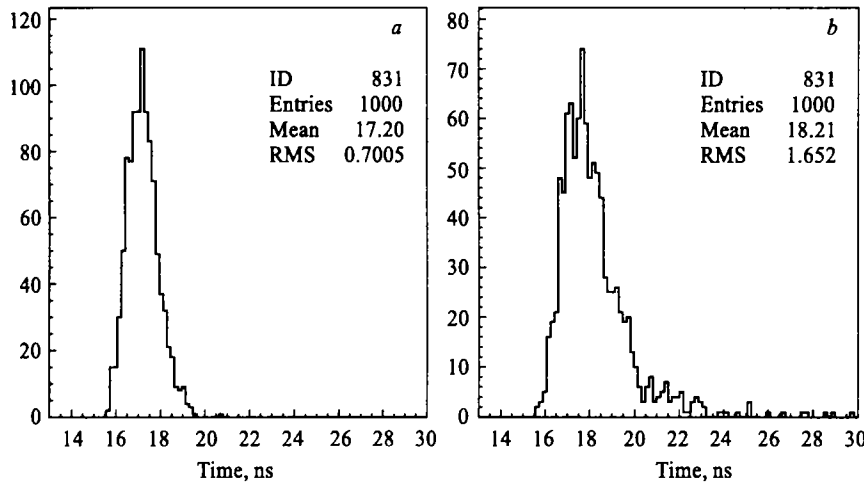
Fig. 4. Distribution of time interval between passage of the particle through the detector and getting signal from the first photon for the detector scheme using the scintillating bar (a) and the bundle of scintillating fibers (b)
