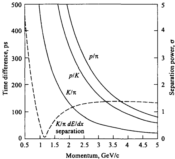
Fig. 1. Time difference as a function of momentum between p/\pi and K/p traversing a distance of 140 cm and separation power assuming a resolution of 100 ps. The dashed line shows the K/\pi separation power from the dE/dx measurement in the Central Outer Tracker
