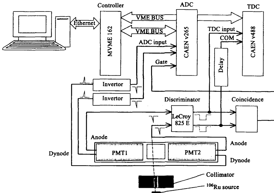
Fig. 5. Construction of the set-up for studying the performance of the Time-of-Flight detector prototypes
