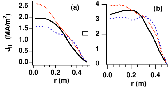
Figure 4. (a) Parallel current density and (b) \bar{q} profiles for times 0.25 ms before (solid), 0.25 ms after (long dash) sawtooth crash, and during PPCD (short dash), generated from MSTFIT equilibrium reconstruction code.
