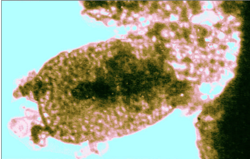
FIG. 1. The transmission electron microscope (TEM) image (magnification 9,000) of an egg-shaped carbon particle of the deposit of type (A). Image width is \sim 750 nm. The internal opaque rod (as a trunk) and the surrounding complicated network of fibers (as a crown) compose a dendrite. The phenomenon of tubularity of structuring is seen in the coaxial tubule, of outer diameter \sim 60 nm, located on the left edge of the particle.
