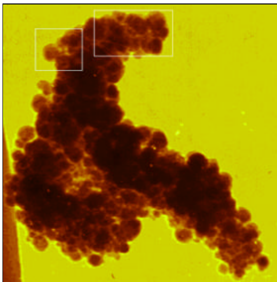
FIG. 4. The TEM image (magnification 26,000) of an agglomerate of visually separate dust particles (deposit of type C; the filter's fiber is partly seen as a dark band on the left hand side of the image). Image width is 590 nm. The magnified images of the windows are given in Figs. 5,6.
