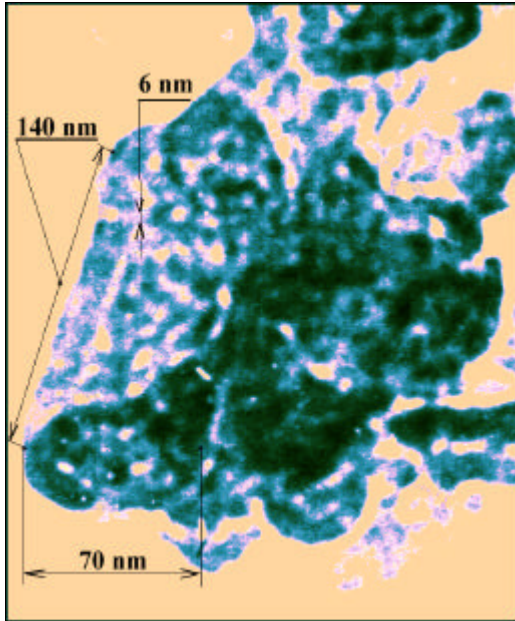
FIG. 2. The TEM image (magnification 34,000) of the fragment of a dust particle \sim 1.2 \mu\text{m} in size (deposit of type B). The tubule whose edge with the distinct central rod is seen in the lower left part of the figure, is of diameter D \sim 70 \text{ nm} and \sim 140 \text{ nm} long. The cylindrical formation ( D \sim 15 \text{ nm} ), which is seen on the left side of the tubule, is its constituent part. The radial bonds between the side-on cylinder and the central rod are of D \sim 5 \text{ nm} .
