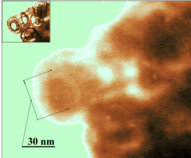
FIG. 5. Magnified image of the window in Fig. 4. The visually separate, quasi-spherical particle appears to be a projection of the edge of a tubular structure ( D \sim 30 nm) which is a part of skeletal structure. For the comments on obtaining a schematic drawing, shown in the left upper corner, see [8(c)].
