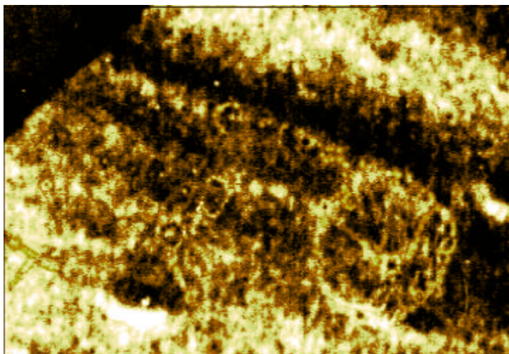
FIG. 7. The scanning electron microscope (SEM) image (magnification 2,000) of the surface layer of the film deposited at the internal surface of the T-10 tokamak chamber. Figure height is \sim 15 \mu\text{m} . Diameter of the tubular structure, whose edge is seen in the right lower part of the Figure, is \sim 5 \mu\text{m} .
