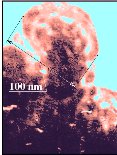
FIG. 3. The image of the cartwheel (all conditions are similar to those of Fig. 2), which is seen on the top of the figure as a wheel ( D \sim 100 \text{ nm} ) declined with respect to figure's plane and connected by radial bonds with a thick vertical formation which is a sort of the axle-tree for this wheel.
