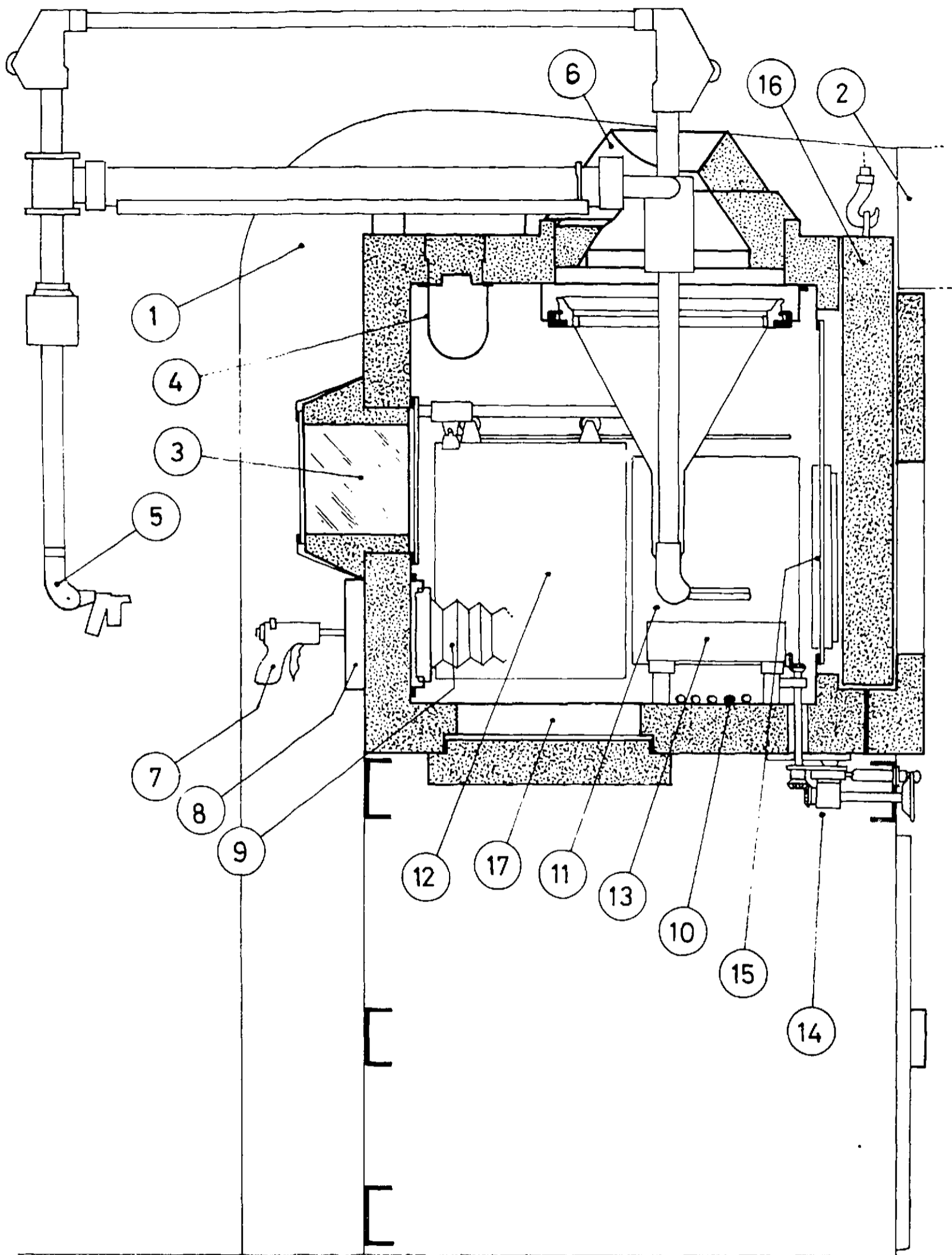
Fig.8. _ CHAINE POLLUX - SAS
