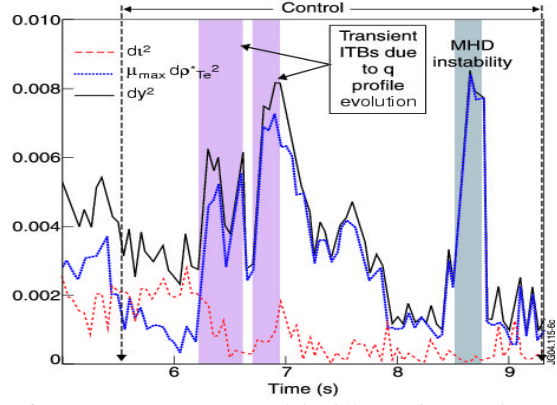
Fig6. Least square minimisation of the difference between the target q -profile (red curve) and its real time measurement (respectively the \rho^*T(x) profile (blue curve)). The sum is given by the black curve.
