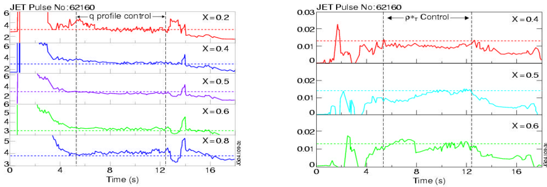
Fig1. Time evolution of the measured and requested q values (a) at 5 radii and \rho^*T values (b) at 3 radii for a controlled pulse (#62160 B_T=3T I_p=1.7MA , current flat top starts at 4s. Dashed lines are set point q and \rho^*_{Te} values. Control starts at 5.5s and stops at 12.3s.
