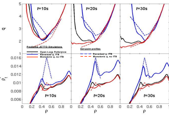
Fig7. Comparison of two closed loop simulations with JETTO for different target q and \rho^*T_e profiles. The picture shows also the open loop reference simulation.
