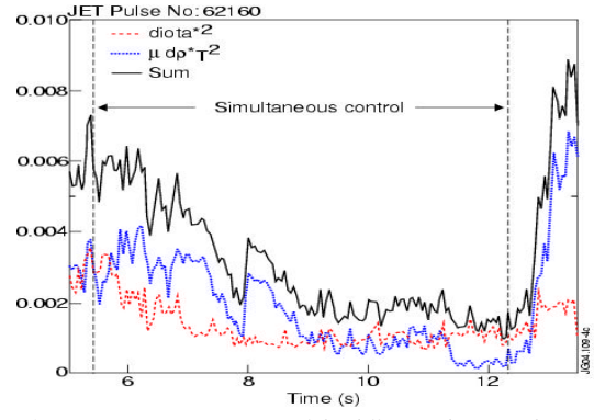
Fig4. Least square minimisation of the difference between the target q -profile (red curve) and its real time measurement (respectively the \rho^*T(x) profile (blue curve)). The sum is given by the black curve.
