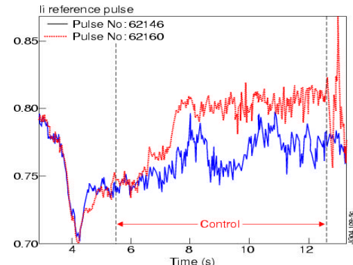
Fig3. Time evolution of the internal inductance of a feedback pulse (#62146, B_t=3T , I_p=1.7MA ) compared to a reference pulse without feedback (#62160, B_t=3T , I_p=1.7MA )
