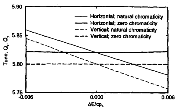
Figure 3: Chromatic tunability with 4-family sextupoles.
