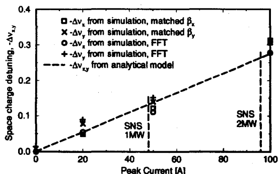
Figure 5: Benchmarking of SIMPSONS simulation.
