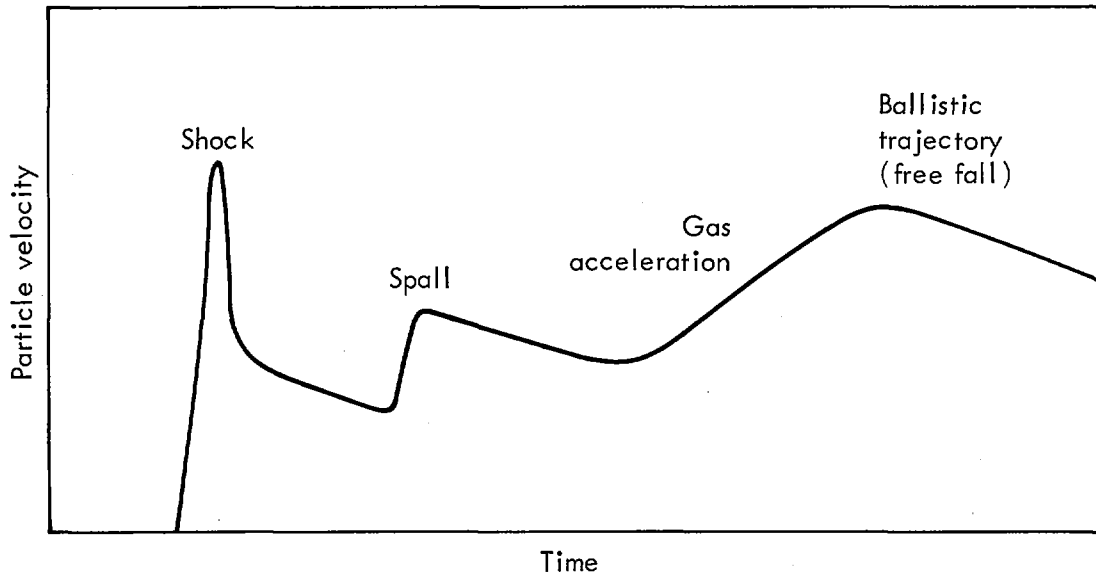
Fig. 1. Cratering mechanisms.
