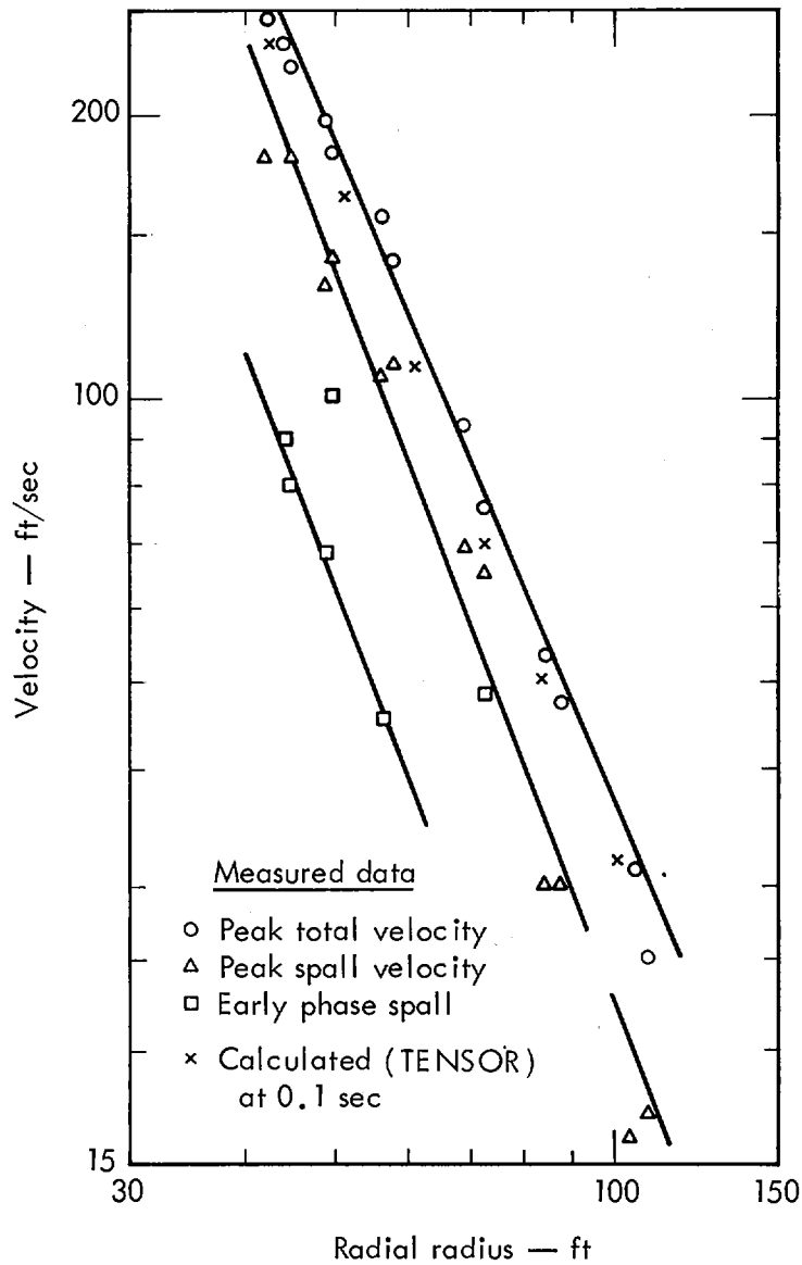
Fig. 13. Surface velocities versus radial range, Pre-Gondola Charley.
