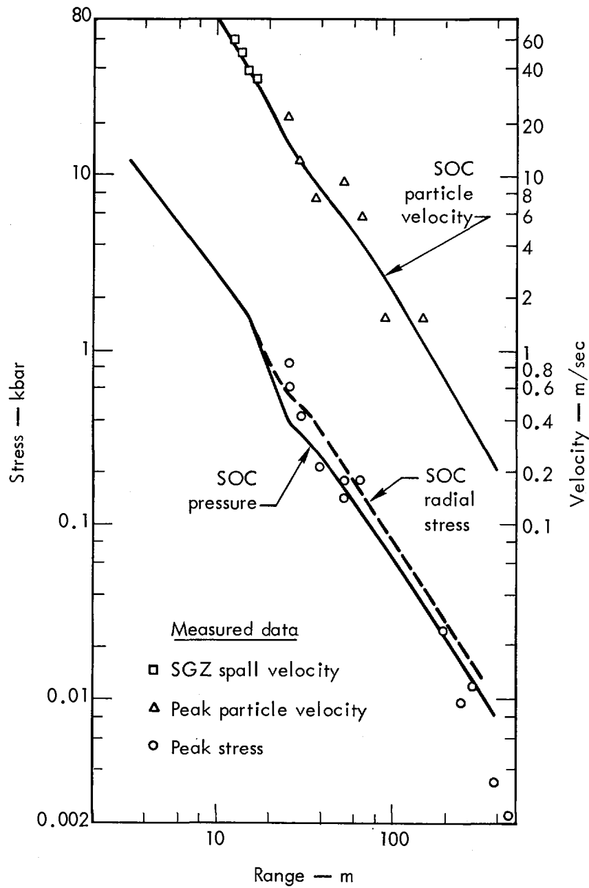
Fig. 12. Peak stress and particle velocity versus range, Pre-Gondola Bravo.
