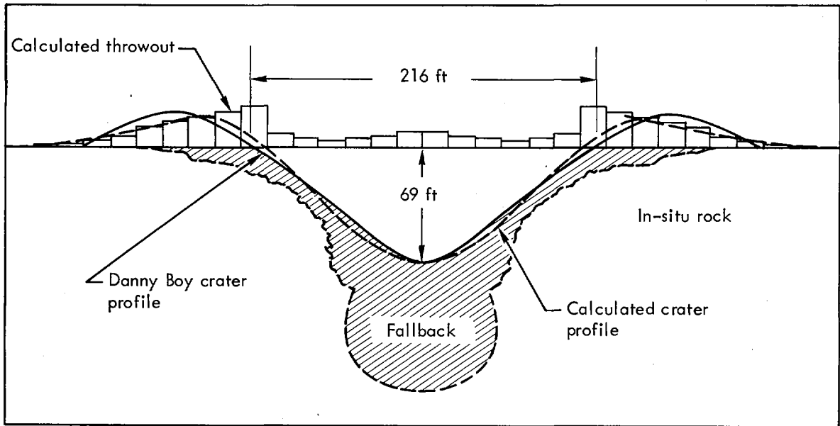
Fig. 20. Calculated crater profile for Danny Boy at t = 0.1 sec.
