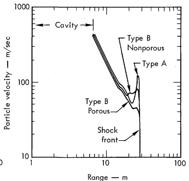
Fig. 5. Particle velocity as a function of compressibility and porosity.
