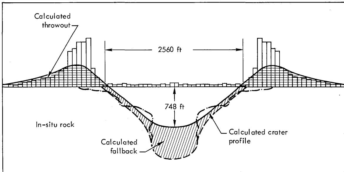
Fig. 25. Calculated crater profile for 1-Mt yield in Divide basalt, 328 m, at t = 3.0 sec.
