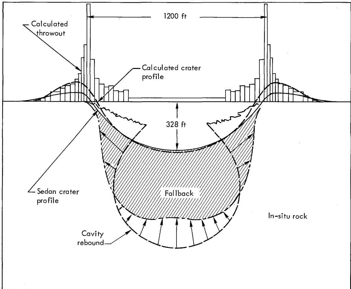
Fig. 17. Sedan crater profile at t = 2.4 sec.
