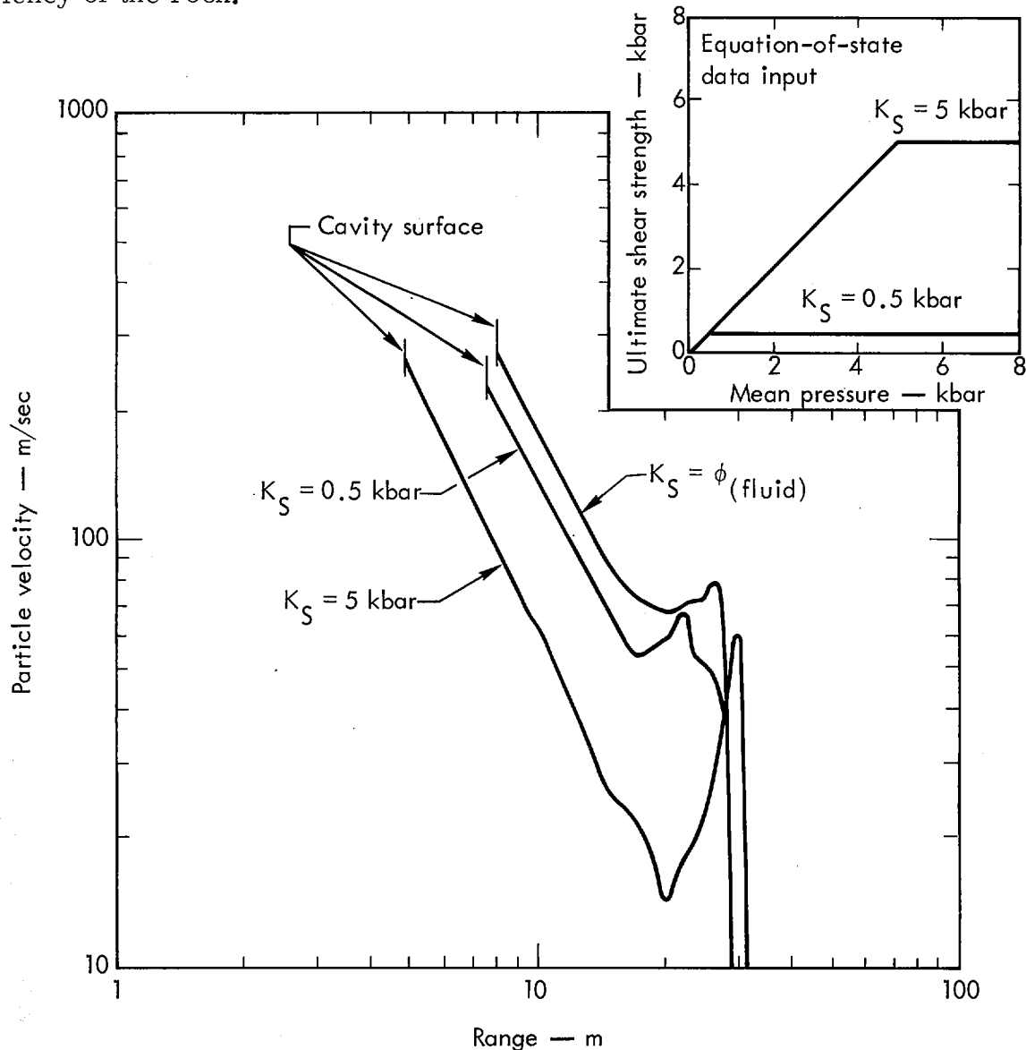
Fig. 6. Particle velocity as a function of shear strength.
