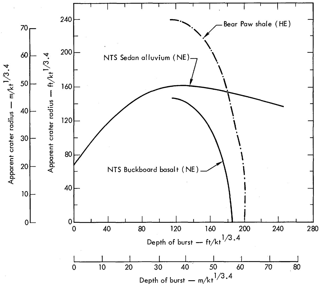
Fig. 9. Scaled crater radius curves.
