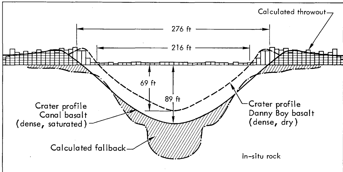
Fig. 23. Calculated crater profile for 0.42-kt yield in Divide basalt, 33 m, at t = 100 msec.
