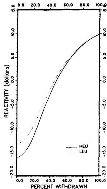
Fig. 2. Reactivity vs Rod Position
