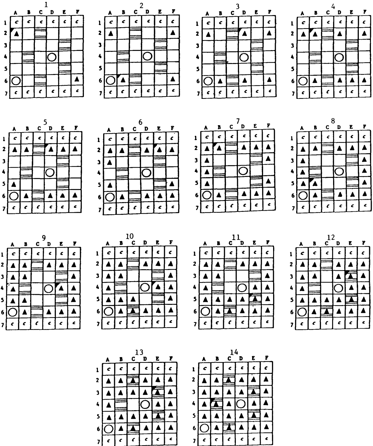
Fig. 3. LEU Replacement Pattern for Each of the Fourteen Cycles Needed To Convert the HEU Core. Triangles Indicate LEU Elements. Tick Mark in Corner Indicates Element With Largest Nuclear Power Peaking Factor.
