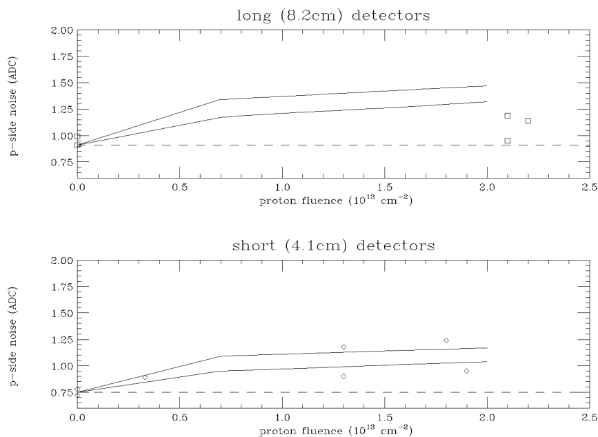
Figure 11: p -side noise versus average radiation dose for the 5 long and 7 short detectors. The solid lines in the figures indicate a range of expected noise as a function of dose. The dotted line indicates the average unirradiated noise value. None of the detectors were believed to have been inverted at the time of the measurements.
