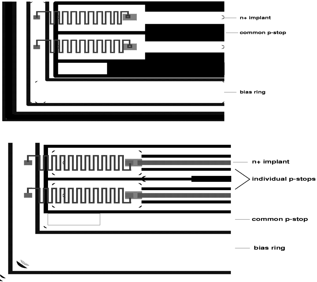
Figure 3: Layout of (top) common and (bottom) combined p -stops
