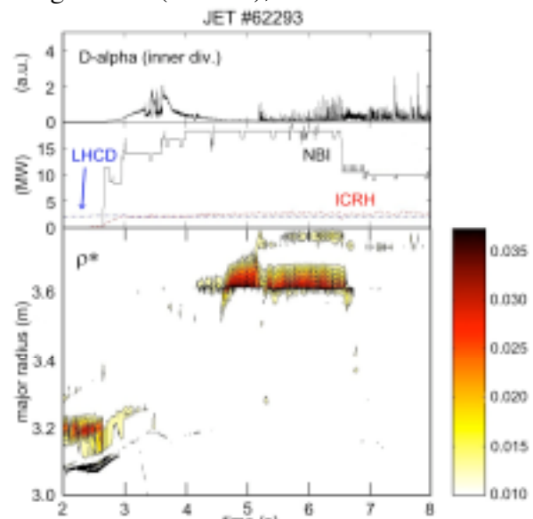
FIG. 1. Contour plot of the strength of a high triangularity ITB, bottom trace), D\alpha , top) and power waveforms, mid trace). The dark area at R \sim 3.7 indicates the position of the barrier very close to H-mode pedestal
