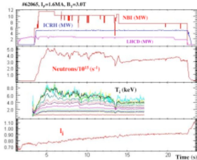
FIG. 5. Time traces of shot 62065, IP=1.6 MA, BT=3.0 T. ITB end at 9s. E=326 MJ inject energy
