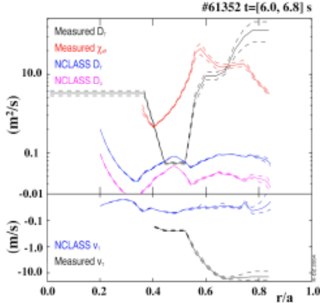
FIG. 7. Measured D_T and V_T (negative inward) compared with neoclassical predictions. Also reported are effective diffusivity and neoclassical prediction for deuterium D
