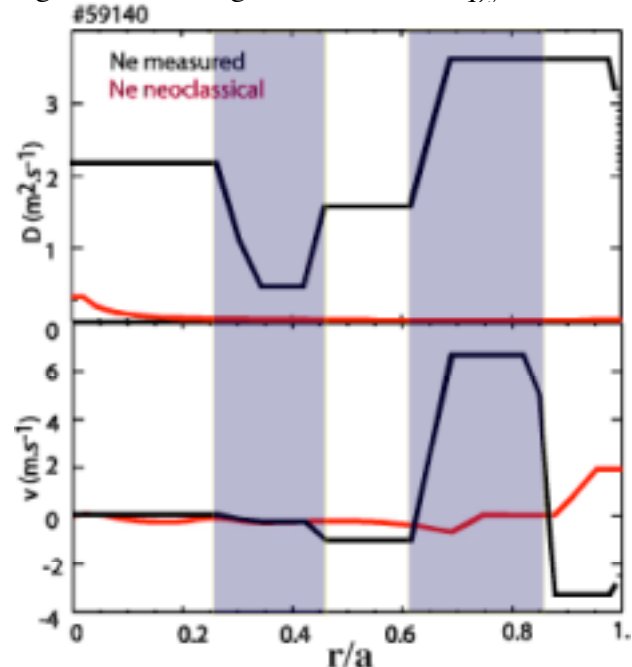
FIG. 8. Measured D (top) and V (Bottom) for Neon in a double barrier. Computed neoclassical values (red lines) are also reported. Shaded areas indicate localisation of barriers.
