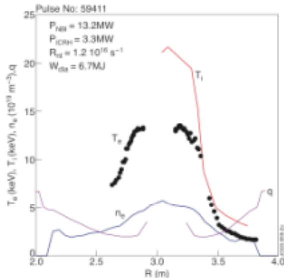
FIG. 6. Temperatures, density and q profiles of a B_T = 3.6 T ITB discharge. 12% ^3\text{He} concentration in D for core deposition of minority and MC ICRF power (33MHz)
