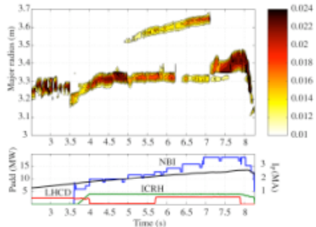
FIG. 2. a) Location of the ITB as a function of time, b) power and I_p waveforms
