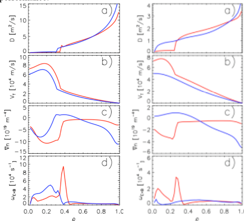
FIG. 4. JETTO simulation: left) #57941 (shallow pellet), right) 55861 (pellet destroying the ITB). Red lines pre-pellet, blue lines post-pellet profiles. a) particle diffusion coefficient, b) plasma toroidal rotation velocity, c) density gradient, d) \omega_{EXB} shear
