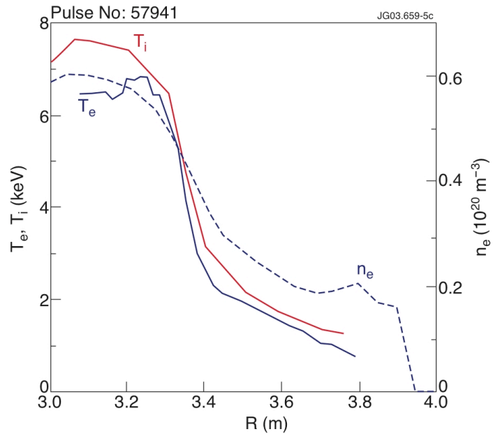
FIG. 3. Density and temperatures profiles of a high density ITB after 1.1 s high power and refuelling with shallow pellets..
