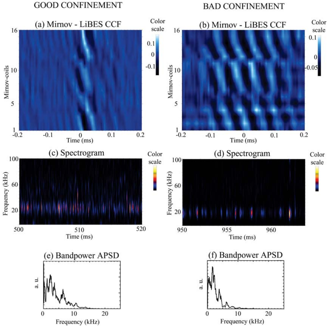
FIG. 2. a) and b) Cross correlation between Li-beam signal and the total Mirnov signals show characteristic undulation with 0.05 time constant, tilted due to delay for different Mirnov-coils and having different relaxation lengths for good and bad confinement. The characteristic undulation is due to main frequency band 20 kHz. c) and d) Spectrograms of Mirnov-coil signals in the processed intervals of shot 47940. e) and f) autospectra of the 15-30 kHz bandpower variations.
