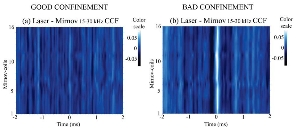
FIG. 4. CCF between the 750 kHz CO_2 laser scattering bandpowers and the bandpower variation of the frequency band 15-30 kHz of the Mirnov-coil signals.
