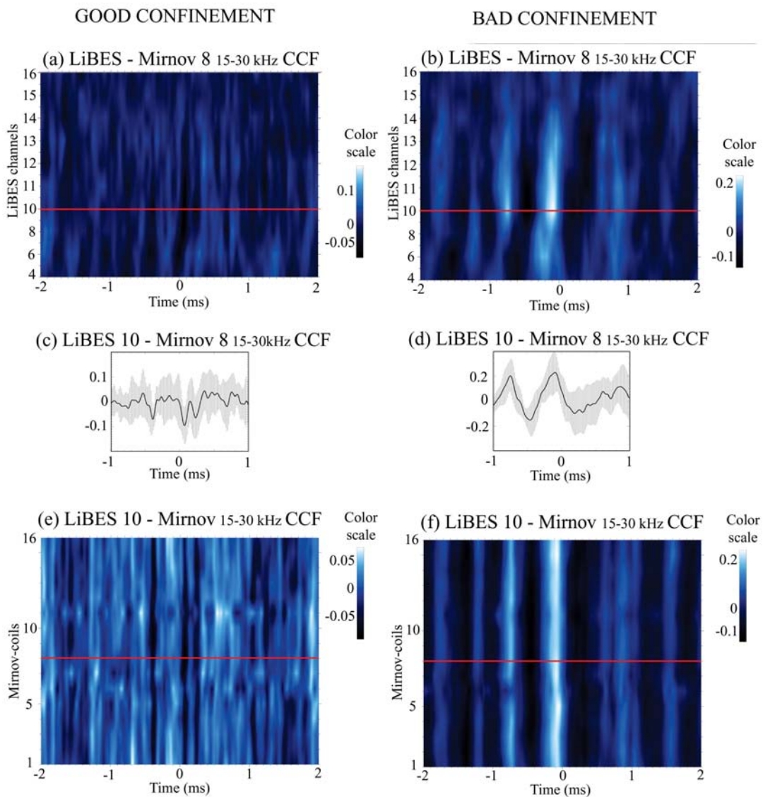
FIG. 3. Cross correlation between the Li-beam signals and the bandpower variation of the frequency band 15-30 kHz of the Mirnov-coil signal. Li-BES channel 4 is in the outer SOL, channel 16 is in the edge plasma.
