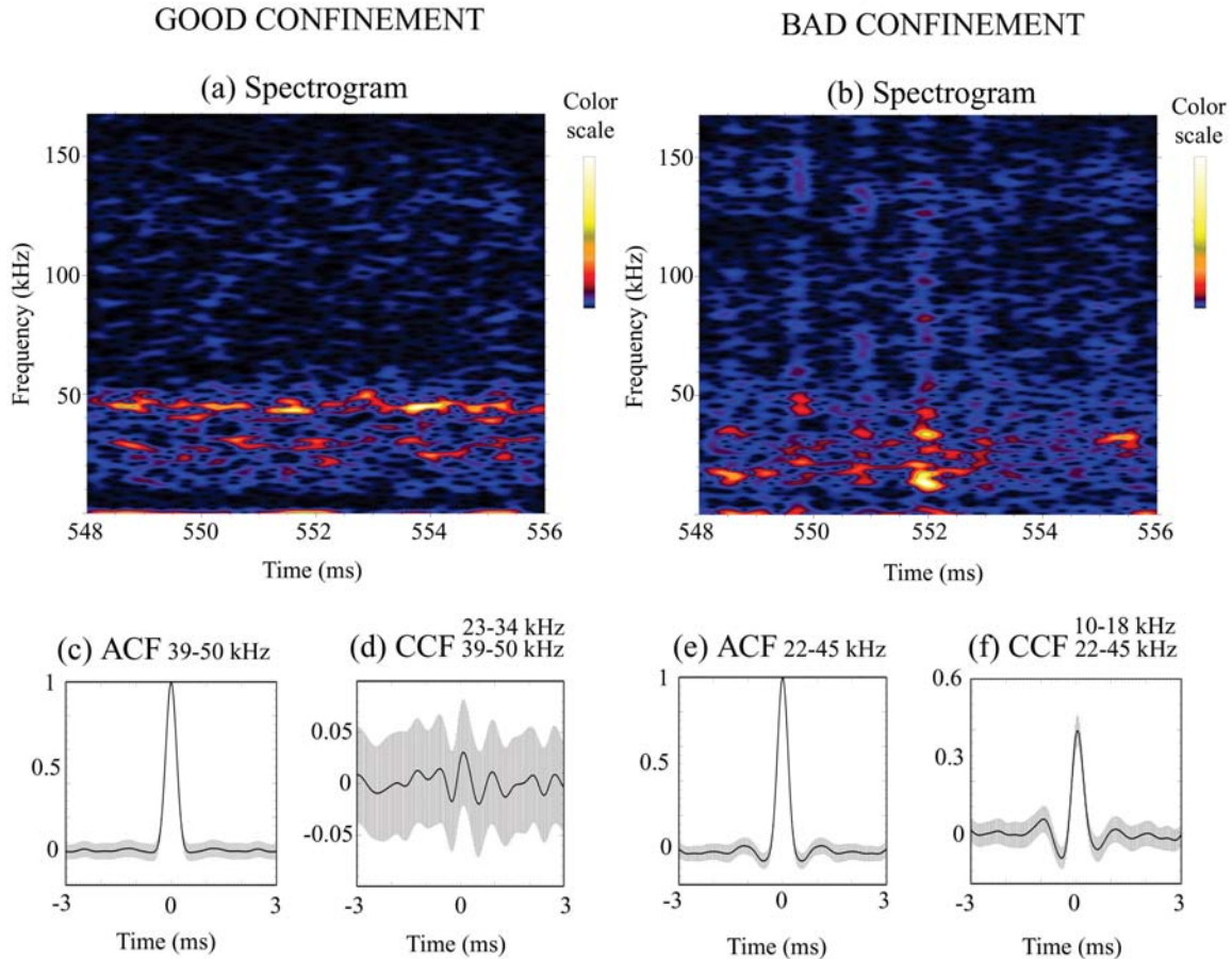
FIG. 1. a) and b) Spectrograms in good and bad confinement states, respectively. c) and e) the ACF of bandpower variation of selected frequency bands (Note, that frequency bands are different in the two cases). d) and f) show the CCF between frequency bands in case of good and bad confinements respectively.
