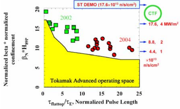
FIG. 7. Progress on NSTX in \beta_N H_{89P} and the plasma flattop time normalized to \tau_E , compared with the equivalent conditions on tokamaks.
