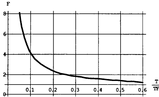
Fig.2. The ratio between the total energy of fermions in the quantum box and in the classical (large) container, F , in function of the ratio of fermion and Fermi temperatures (when T/T_F \ll 1 ).
