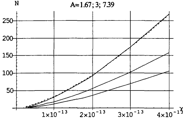
Fig.1. The plot of the number of particles in Fermi-Dirac gas, N , versus the adiabatic invariant multiplied by the atomic mass number, \gamma = A_{at} L^2 T [ \text{cm}^2 \cdot \text{K} ], at fixed fugacity, A , using direct summation (continuous lines, from bottom to top: A = 1.67, 3 and 7.39 ) and the integral approximation from Eq.(17) (for A = 7.39 , dashed line). The value A = 1.67 is close to the onset of quantum regime, while A = 7.389 is close to the lowest experimental limits.
