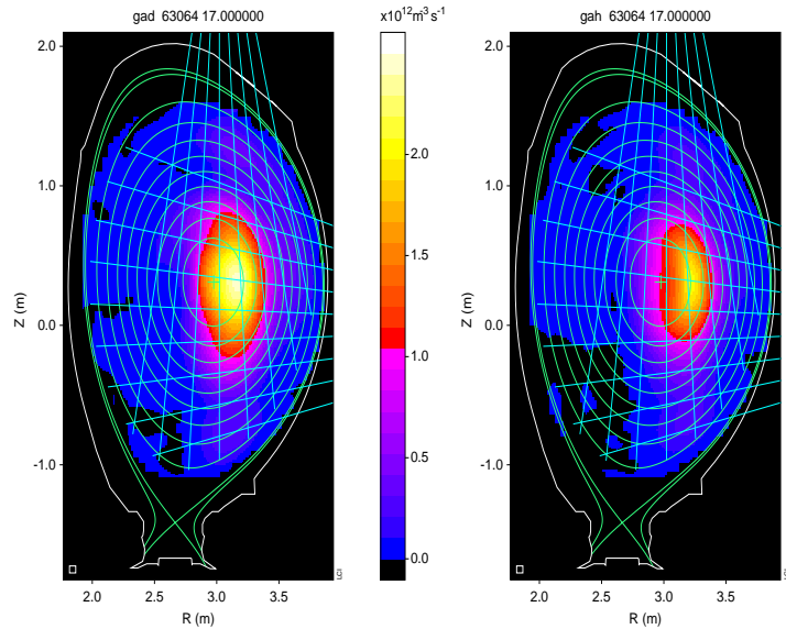
FIG. 3. Gamma-ray images of \alpha particles and D-ions measured simultaneously during a 2.2 T/2.0 MA JET discharge with ICRH heating: with in plasmas: left - D-image ( E_D > 0.8 MeV); right - alpha-image ( E_\alpha > 1.7 MeV)
