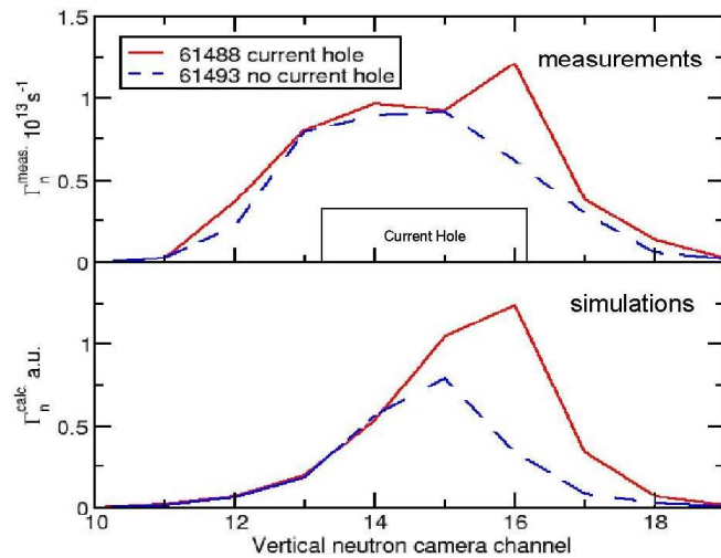
FIG. 2. Comparison of 14 MeV neutron profiles for on-axis tritium beams (measured at the top, calculated at the bottom). An outward displacement of neutron emission is clearly seen for plasmas with a current hole.
