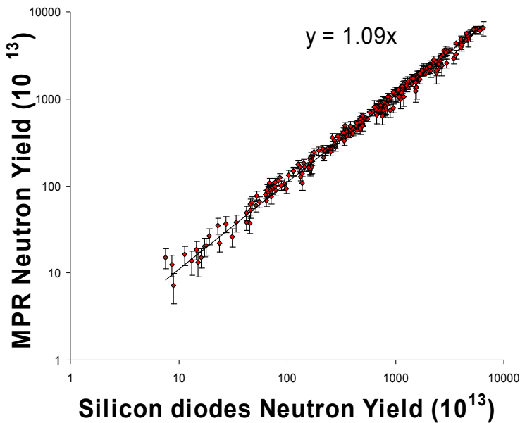
FIG. 1. Cross validation of the 14 MeV neutron yield measurements for the TTE campaign. The deviation from a 1:1 proportionality is within the errors of the two diagnostics.
