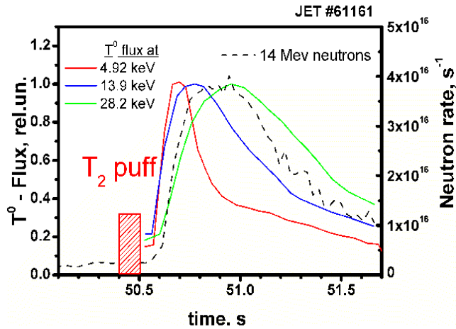
FIG. 4. Escaping neutral tritium fluxes measured by the NPA.
