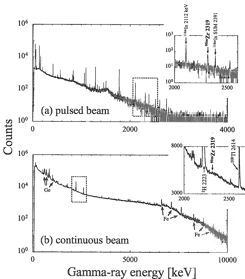
Fig. 3. Gamma-ray spectra of ^{90}\text{Zr}(n, n')^{90\text{m}}\text{Zr} reaction measured with the pulsed neutron beam (a) and the continuous neutron beam (b).
