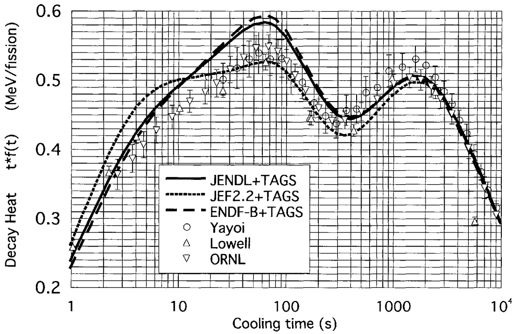
Fig. 2 Decay heat after a burst fission in Pu-239 after the TAGS correction (γ-ray component)
