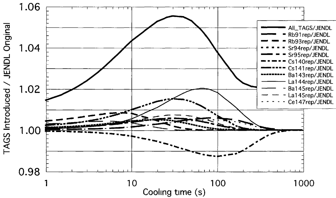
Fig. 3 Effect of introduction of TAGS energies into JENDL summation calculation (fast fission in Pu-239, γ-ray component)
