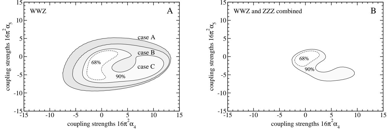
Figure 2: Expected sensitivity for \alpha_4/\alpha_6 and \alpha_5/\alpha_7 at \sqrt{s} = 1000 GeV. Luminosity assumption 1000 \text{ fb}^{-1} . A) WWZ-channel only, for an unpolarized beam (A) and the different polarizations cases, e^- only polarized (B) and both beams polarized (C) as explained in the text. Solid lines represent 90% confidence level, the dashed line is for 68%, i.e. \Delta\chi^2 = 2.3 . B) Combined fit using WWZ of case C and ZZZ production. Lines represent 90% (outer line), 68% (inner line) confidence level.
