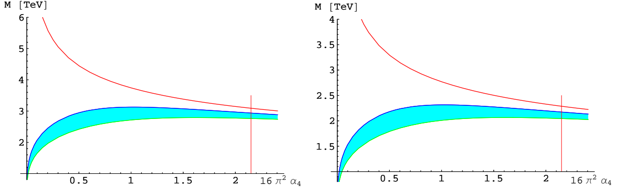
Figure 17: Dependence of the resonance mass for the charged component of the vector triplet on \alpha_4 for different assumed widths ( f=1 on the left and f=0.3 on the right) for g = -h case, but \ell_\rho, \ell'_\rho \neq 0 . The red and blue line are the lower and upper limit from \lambda_Z , respectively. Vertical red line: maximal allowed value of \alpha_4 . The blue shaded area is the allowed one when \mu_\rho, \mu'_\rho \neq 0 .
