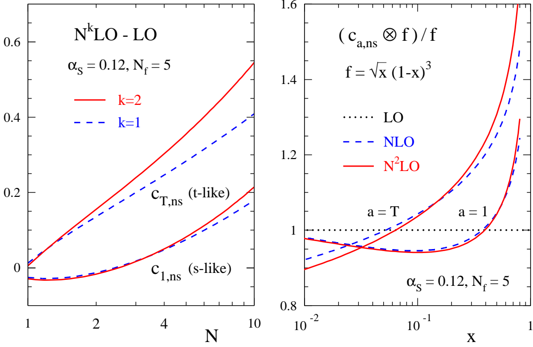
Figure 1: Comparison of the coefficient function c_{T,ns} for the (time-like) process e^+e^- \rightarrow h+X with its counterpart c_{1,ns} in (space-like) deep-inelastic scattering for Q^2 \simeq M_Z^2 . Left plot: Mellin moments, right plot: convolutions (2) with a schematic input shape denoted by f .
