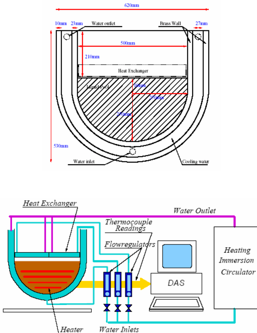
Figure 1. The schematic of the SIMECO test section and test facility.
