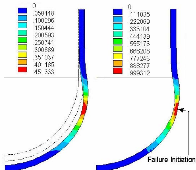
Figure 6. Distribution of the equivalent creep strain (left, max. 0.45) and the damage (right, max. 0.9993) at calculated failure time of t = 4:05\text{h} (38 kW, 25 bar, Experiment EC2). ANSYS calculations were performed by H. Willschuetz et al. , using the KTH-developed ECCM (effective-conductivity-convectivity model) model for simulation of natural convection heat transfer in volumetrically heated melt pools.
