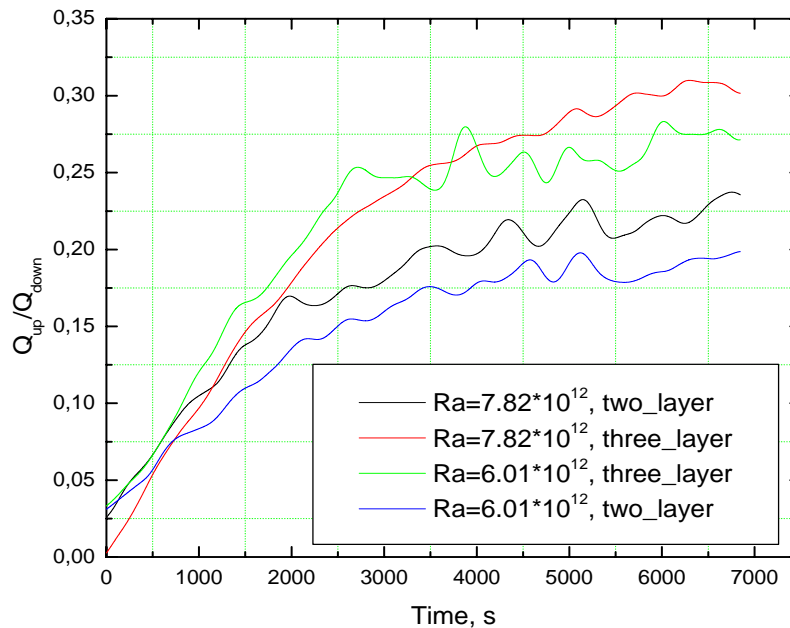
Figure 2. Q_{up}/Q_{down} ratio in SIMECO two- and three-layers experiments.
