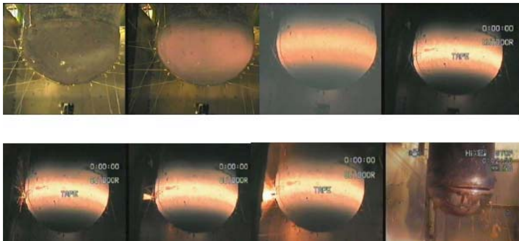
Figure 4. Photographs of the sequence of the EC FOREVER-4 test.
