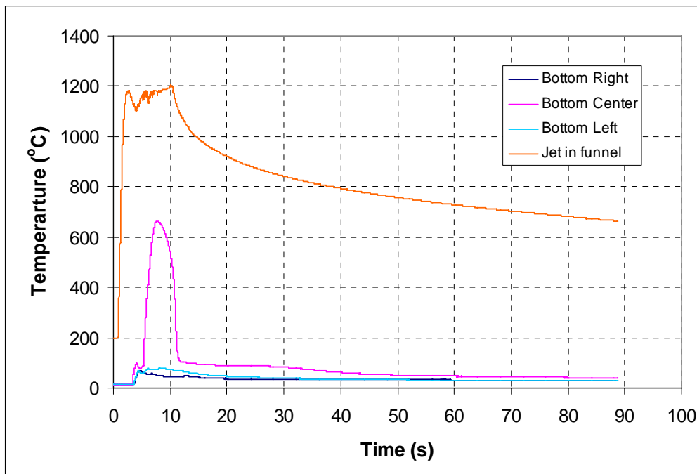
Figure 12. Temperature as measured by thermocouples in the funnel nozzle, and in the tank bottom. The bottom center thermocouple shows that the debris settled is initially unquenched (debris surface's temperature is higher than Leidenfrost temperature). Later quenching of the debris region surrounding the thermocouple occurred before melt pour was completed, indicating that the cooling and quenching were due to water ingress from the side.
