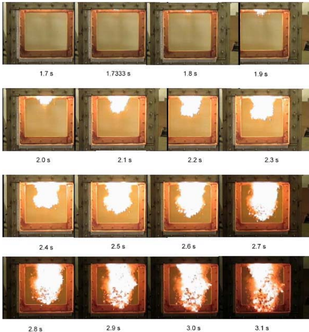
Figure 13. DEFOR-1 test: Fragmentation of a high-temperature binary-oxidic melt jet in a subcooled water pool, with subsequent intense debris-coolant mixing and heat transfer, and formation of a high-porosity debris bed on the tank bottom.
