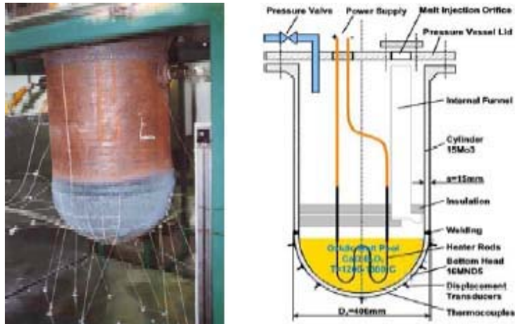
Figure 3. The FOREVER facility: a 1/10th scale (400mm diameter, 15mm wall thickness) carbon steel vessel, constructed, welded, and heat-treated according to the vessel manufacture code. The experiment is performed by pouring a binary oxide (CaO-B 2 O 3 ) melt of about 12 liters at 1200°C into a scaled reactor pressure vessel, heating the melt to maintain temperature level at 1100 to 1200°C, and pressurizing the vessel wall up to 25 bars pressure with Argon gas. The vessel wall temperature reached 800 to 1000° and the vessel experienced creep and eventually failure.
