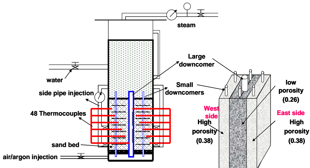
Figure 10. The schematic of POMECO test section (left) and a configuration of particulate bed with downcomers (right).
