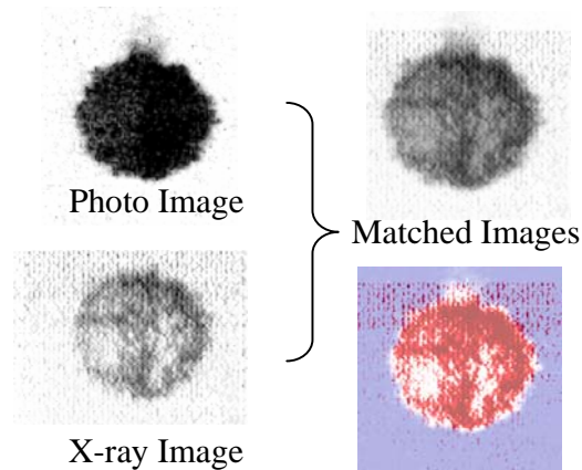
Figure 15. The SHARP images for a highly-superheated molten tin drop steam explosion.
