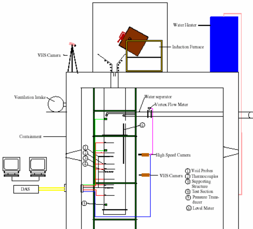
Figure 11. The schematic of the DEFOR facility (previously MIRA-20L). High-temperature (superheated) binary-oxide melts are poured into a water tank (of different depths, and different subcoolings). The tank sidewalls are made of Plexiglas to allow visualization of jet breakup and debris formation.
