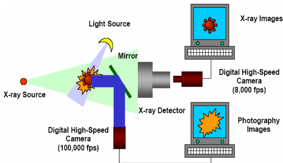
Figure 14. The SHARP system in the MISTEE facility.
