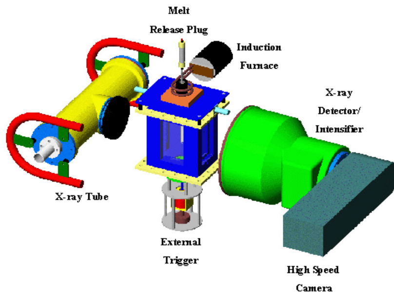
Figure 13. The MISTEE facility.
