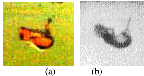
Figure 16. MnO-TiO 2 melt drop (~1400 °C) in water: (a) photograph image and (b) X-ray image.
