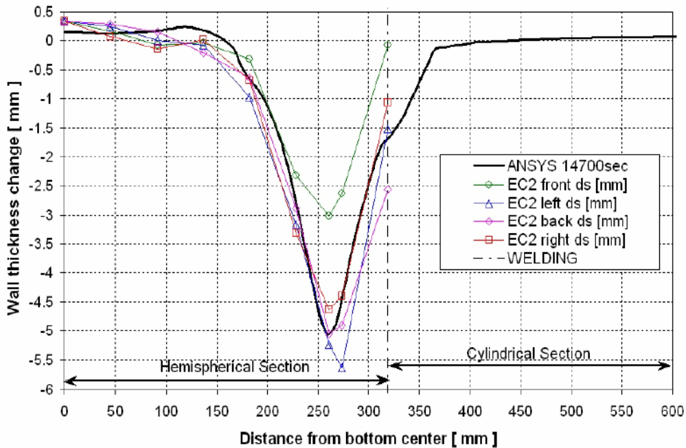
Figure. 7. Wall thickness change along the meridian line of the vessel at failure time (FOREVER-EC2 experiment). ANSYS calculation by H. Willschuetz.
