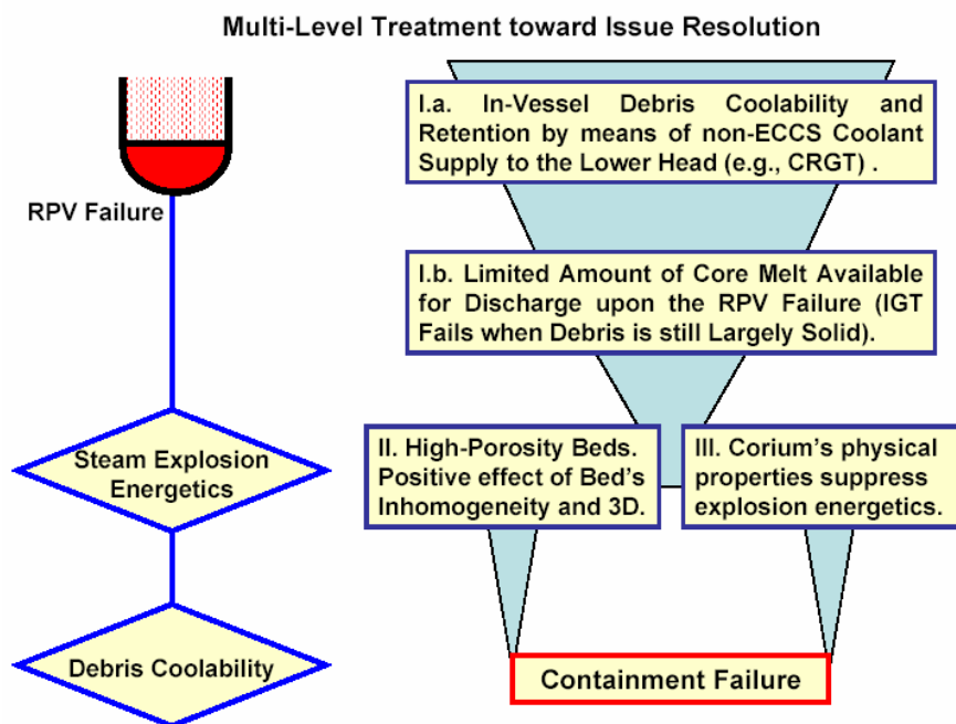
Figure 17. The connection between KTH research and quantification of risk of containment failure. KTH research addresses “limiting” mechanisms. Except for I.a (which calls for a mitigative measure), the others (I.b, II and III) aim to establish and exploit the hidden margins.
