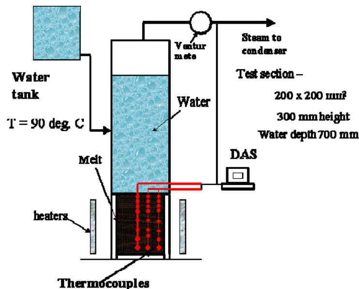
Figure 8. The schematic of COMECO facility
