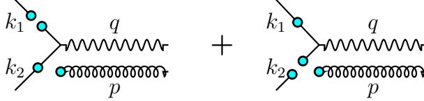
Figure 4: Instanton-induced process for n_f = n_g = 1 , q_L(k_1) + \bar{q}_L(k_2) \rightarrow \gamma^*(q) + g(p) , in leading semiclassical approximation.
