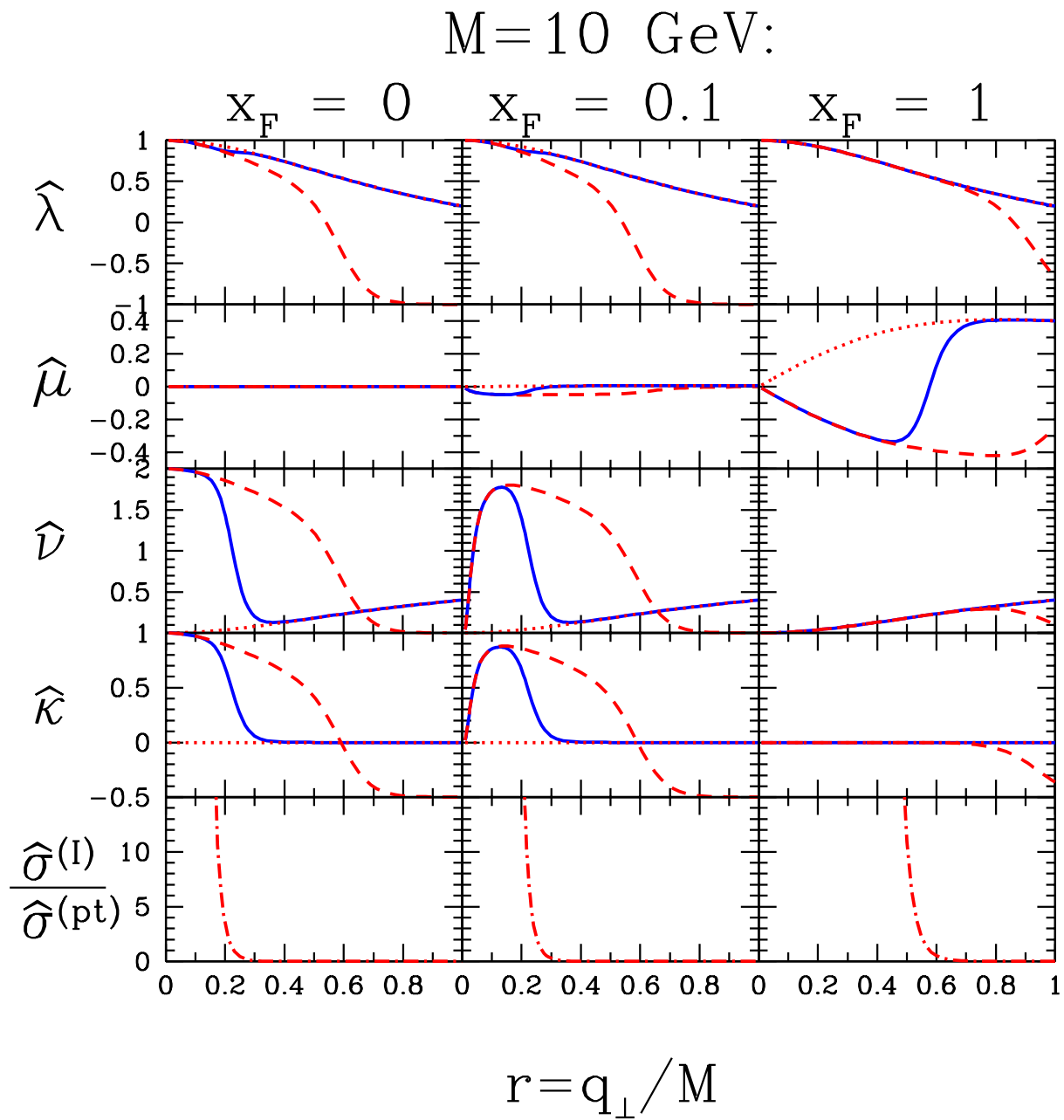
Figure 6: Same as in Fig. 5, but for M = 10 GeV.
