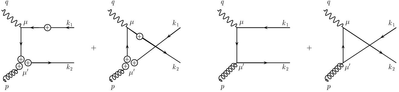
Figure 3: Instanton-induced process for n_f = n_g = 1 , \gamma^*(q) + g(p) \rightarrow \bar{q}_R(k_1) + q_R(k_2) , in leading semiclassical approximation (left) and the analogous process, \gamma^*(q) + g(p) \rightarrow \bar{q}_R(k_1) + q_L(k_2) , from ordinary perturbation theory (right). Both figures from Ref. [12].
