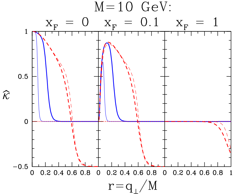
Figure 7: Illustration of the dependence of our prediction of the Lam-Tung parameter \hat{\kappa} = \frac{1}{4}(1 - \hat{\lambda} - 2\hat{\nu}) on the choice of n_f and \Lambda , for fixed M = 10 GeV and various values of x_F . The thicker lines correspond to our default choice n_f = 3 and \Lambda = \Lambda_{\overline{\text{MS}}}^{(3)} = 0.346 GeV, whereas the thinner ones correspond to n_f = 1 and \Lambda = \Lambda_{\overline{\text{MS}}}^{(1)} = 0.241 GeV (other notations as in Figs. 5 and 6).
