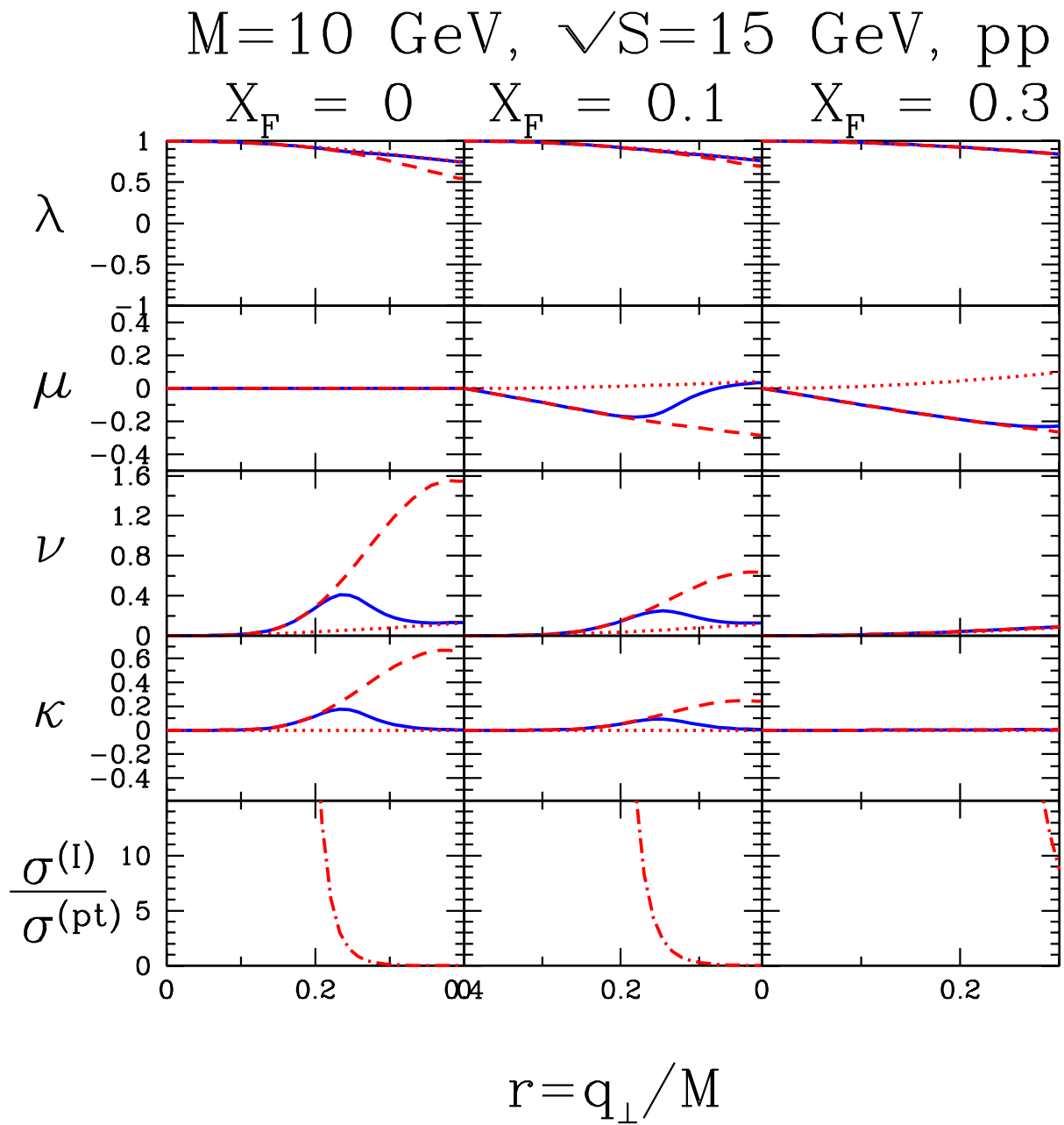
Figure 9: Same as in Fig. 8, but for M = 10 \text{ GeV} .
