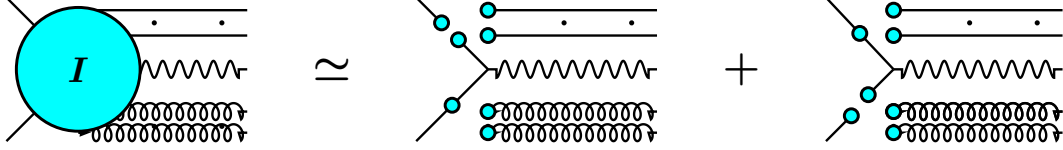
Figure 2: Instanton-induced process for n_f = 3 , u_L + \bar{u}_L \rightarrow \gamma^* + \bar{d}_R + d_R + \bar{s}_R + s_R + n_g g , in leading semiclassical approximation. The amplitude involves the products of the appropriate classical fields (lines ending at blobs: fermionic zero modes (straight) and instanton gauge fields (curly)) as well as the non-zero mode quark propagator in the instanton background (quark line with central blob).
