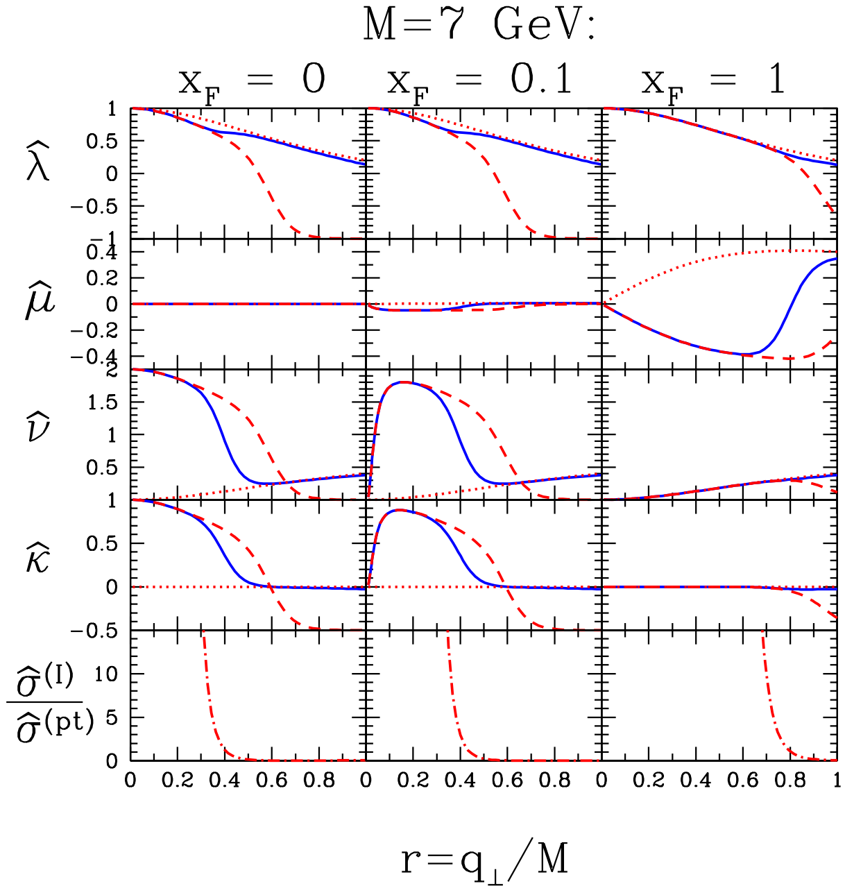
Figure 5: Coefficient functions of the angular distribution of lepton pairs from quark anti-quark annihilation, as a function of q_{\perp}/M , for various values of x_F , for M = 7 \text{ GeV} . Dotted: result from pure ordinary perturbation theory; dashed: result from pure instanton perturbation theory; solid: total result from ordinary and instanton perturbation theory. Also shown, in the last row, is the ratio of the cross-sections of instanton perturbation theory to ordinary perturbation theory (dashed-dotted). In the numerical results shown we have chosen \mu_r = M , \Lambda = 0.346 \text{ GeV} , and n_f = 3 .
