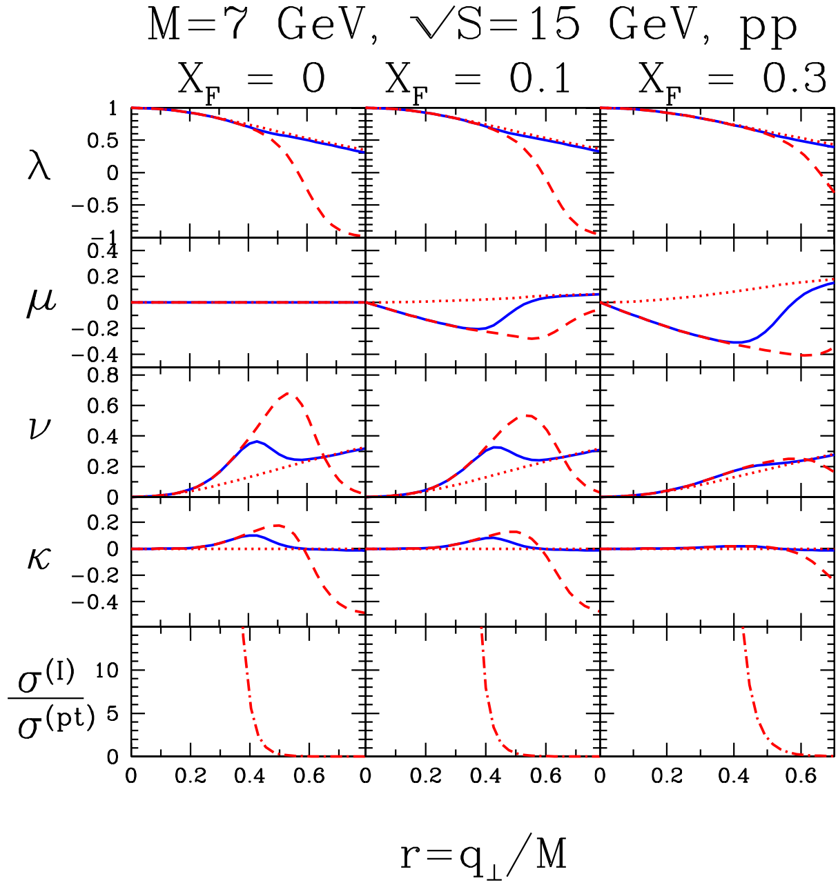
Figure 8: The plot shows the angular structure functions similar to Fig. 5 but on hadron level. Therefore an integration over parton distributions, e.g. for the proton, is included. Due to the variable momentum fractions x_1 and x_2 one has to specify an additional kinetic variable, e.g. the c.m. energy \sqrt{S} .
