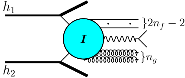
Figure 1: QCD instanton-induced contribution to lepton pair production in hadron-hadron collisions, h_1 + h_2 \rightarrow (n_f - 1) [\bar{q}_R + q_R] + \ell^+ + \ell^- + n_g g + X , corresponding to n_f light flavours.
