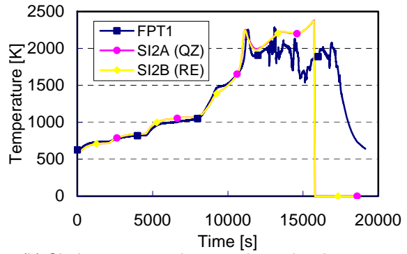
(b) Clad temperature in outer ring at level 600 mm.
