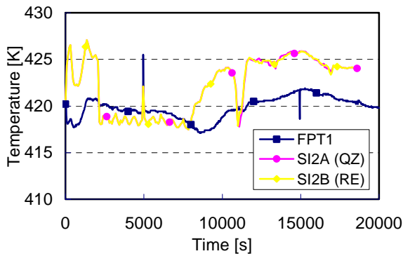
(g) Cold leg fluid temperature.
