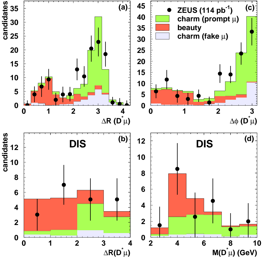
Figure 5: Distributions of (a) \Delta R(D^*\mu) , (c) \Delta\phi(D^*\mu) for unlike-sign events in the inclusive sample, (b) \Delta R(D^*\mu) and (d) M(D^*\mu) for for unlike-sign events in the DIS sample after subtraction of the fake- D^* background. Data points (full circles) are shown together with the fitted contributions from beauty and charm, as indicated in the legend. The fake-muon contribution from charm is shown separately, but fitted together with the charm contribution.
