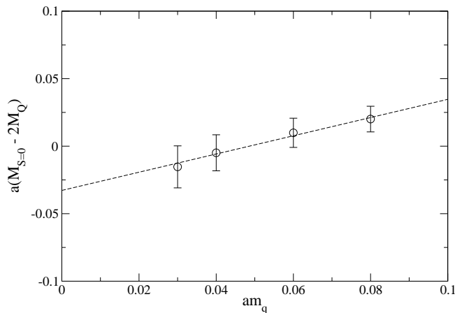
FIG. 8: Difference between the effective mass of the scalar diquark and twice the constituent quark mass, as a function of bare quark mass.
