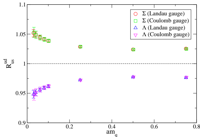
FIG. 6: Ratios of RMS quark separations as a function of bare quark mass am_q .
