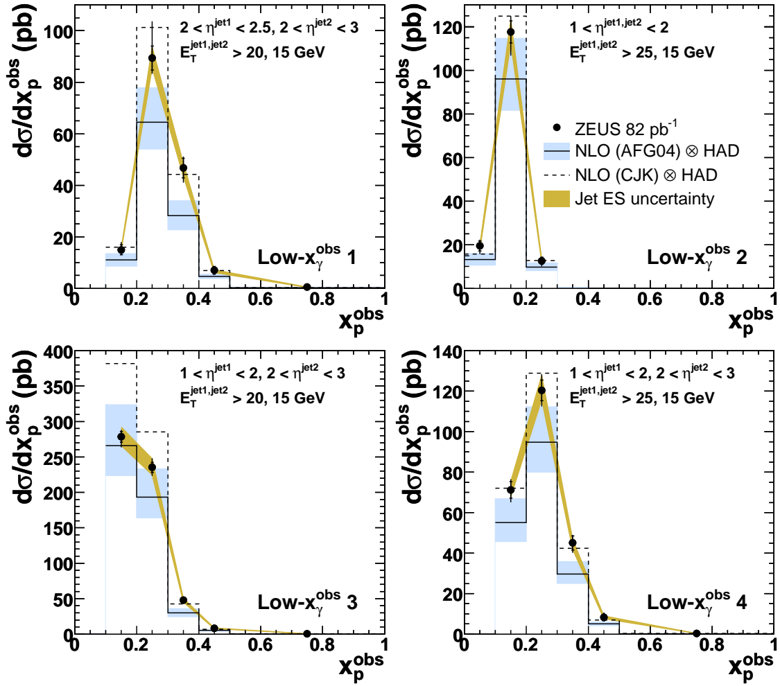
Figure 10: Optimised cross-sections d\sigma/dx_p^{\text{obs}} for x_\gamma^{\text{obs}} \leq 0.75 in the kinematic regions defined in Table 1. For further details, see the caption to Fig. 4.
