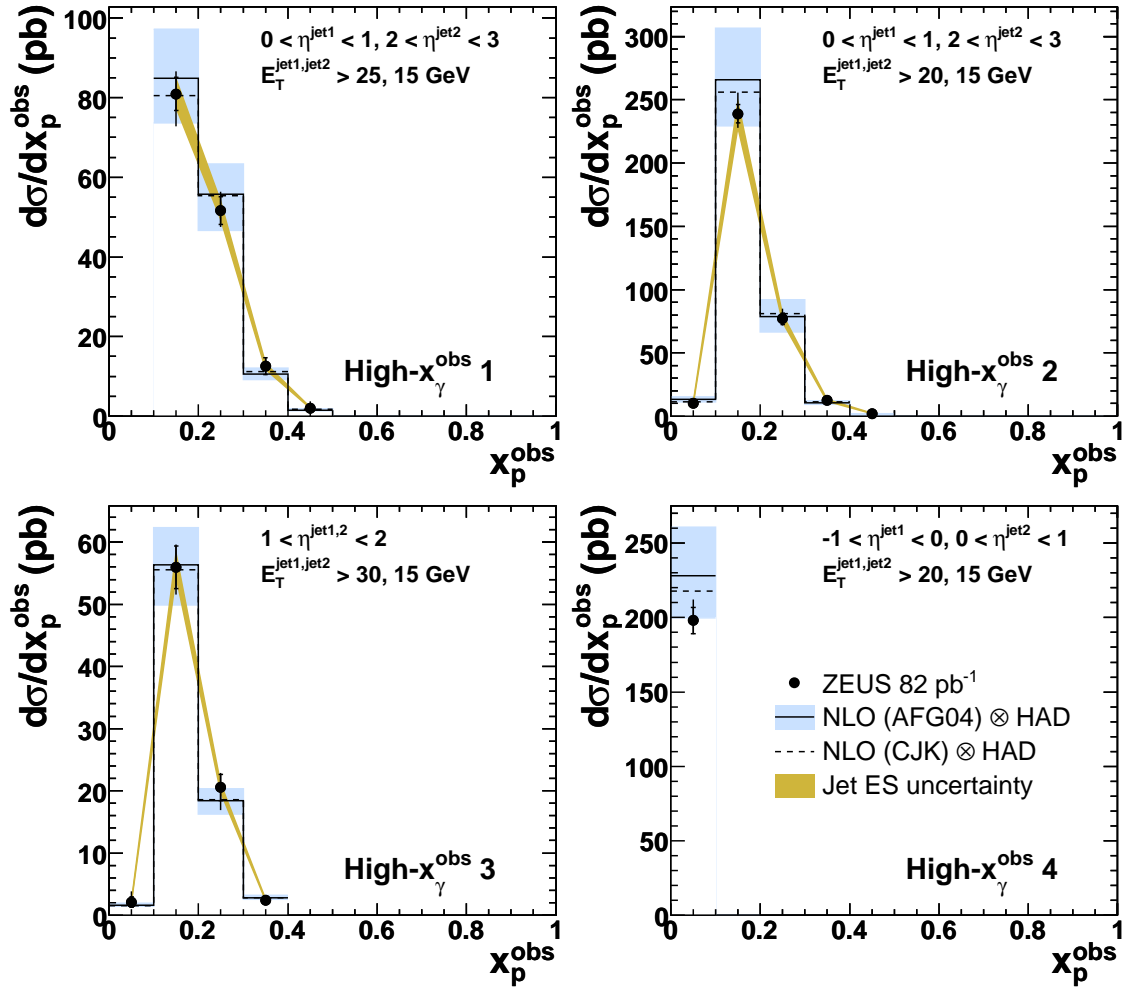
Figure 9: Optimised cross-sections d\sigma/dx_p^{\text{obs}} for x_\gamma^{\text{obs}} > 0.75 in the kinematic regions defined in Table 1. For further details, see the caption to Fig. 4.
